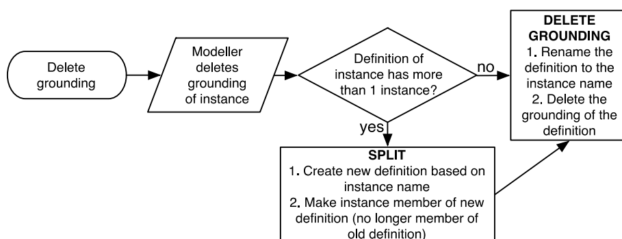
Figure 13: Flow diagram showing the procedure when deleting groundings of instances.
