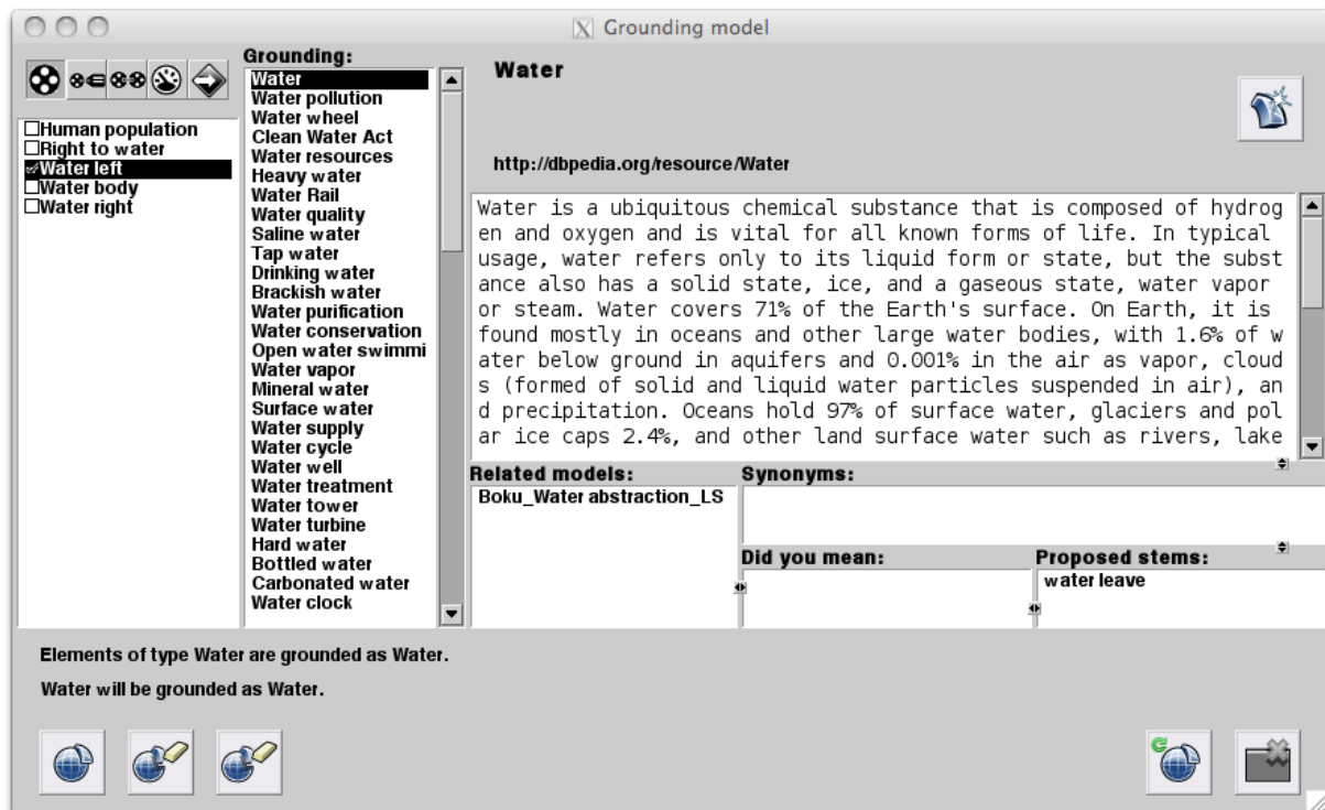
Figure 11: The grounding dialog adapted for instances.
