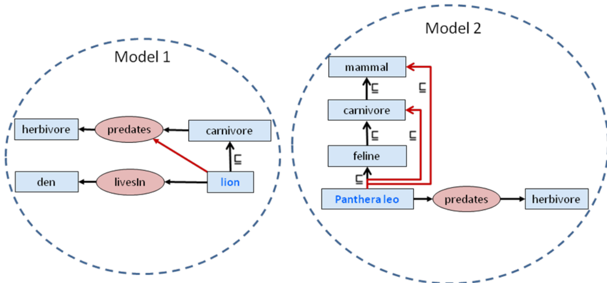
Figure 4: models with new inferred facts
