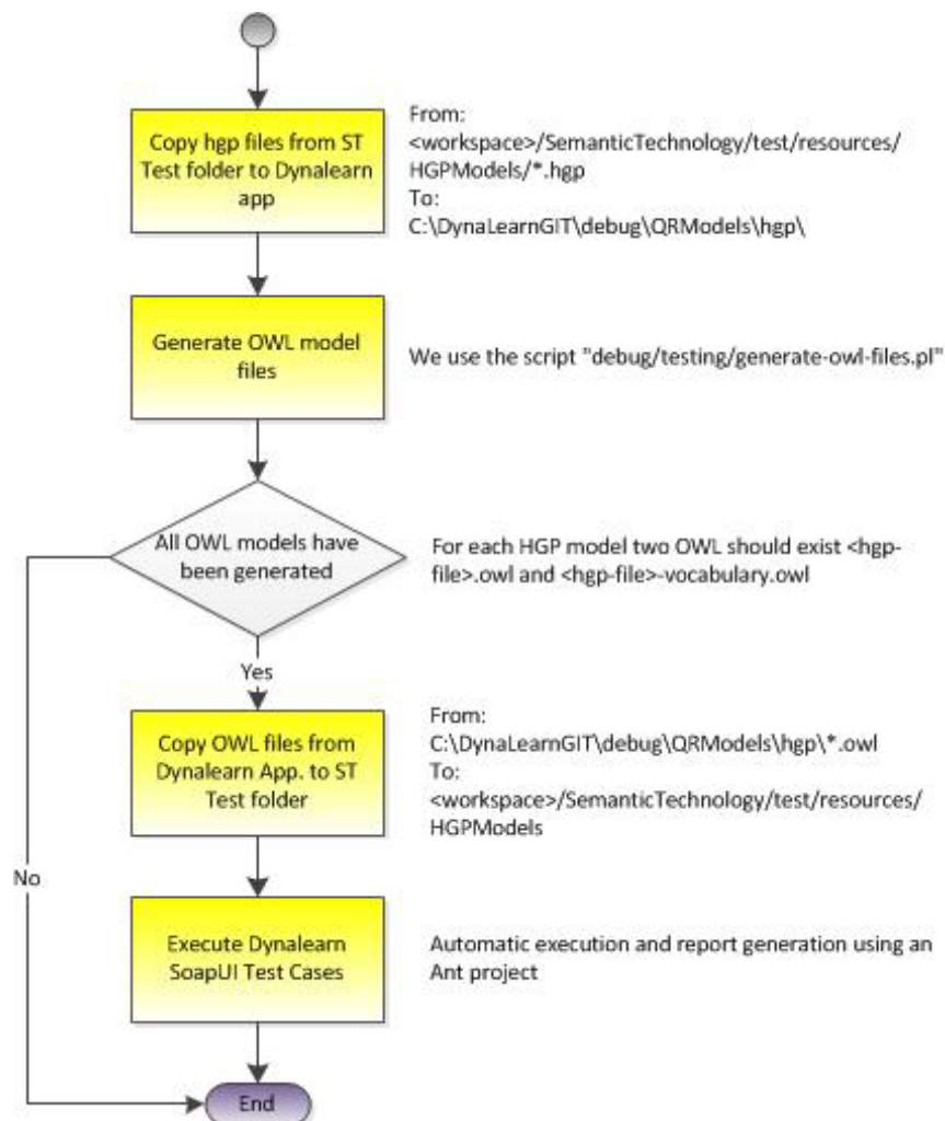
Figure 14: Flowchart of the testing process
