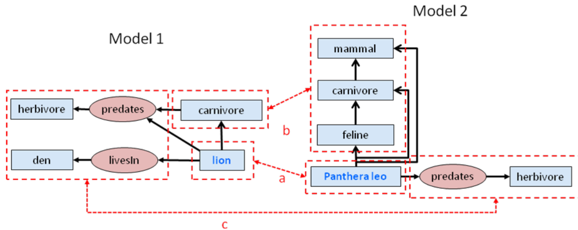
Figure 5: comparisons between the inferred ontologies
