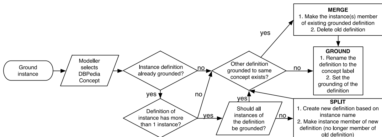
Figure 12: Flow diagram showing the procedure followed when grounding instances.
