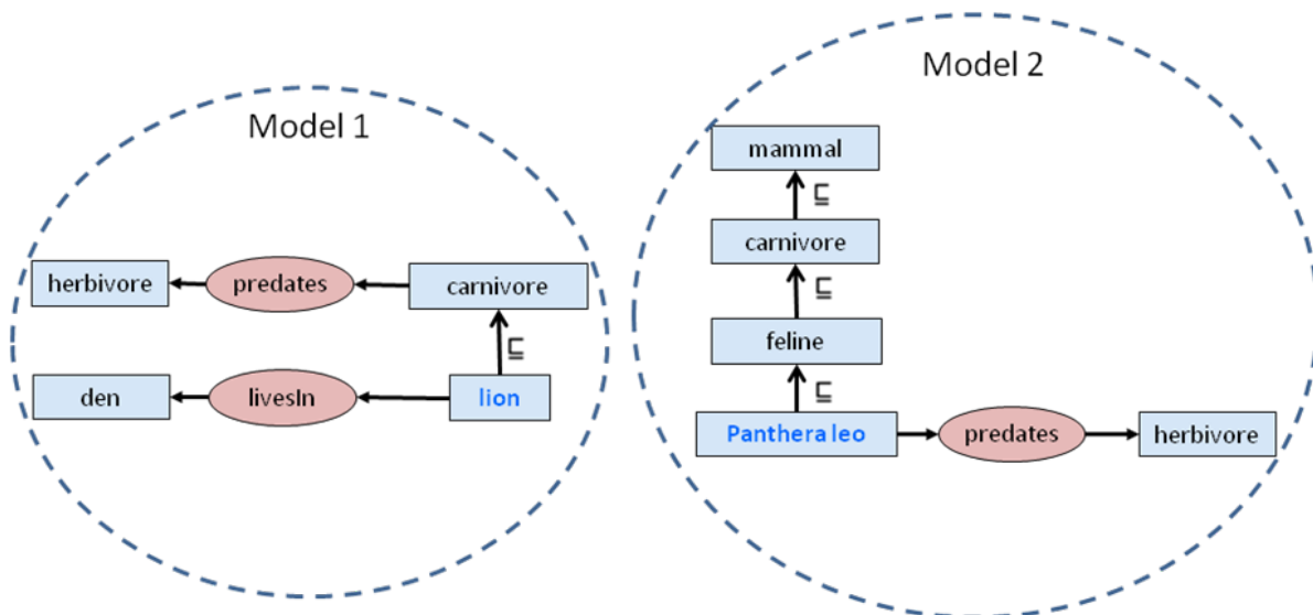
Figure 2: example of models to be matched ( \sqsubseteq denotes subsumption)
