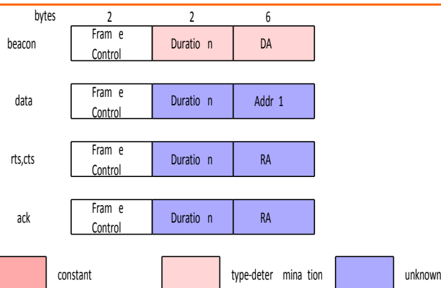
Figure 4-10: Fields considered by the reliable frame type estimator.
