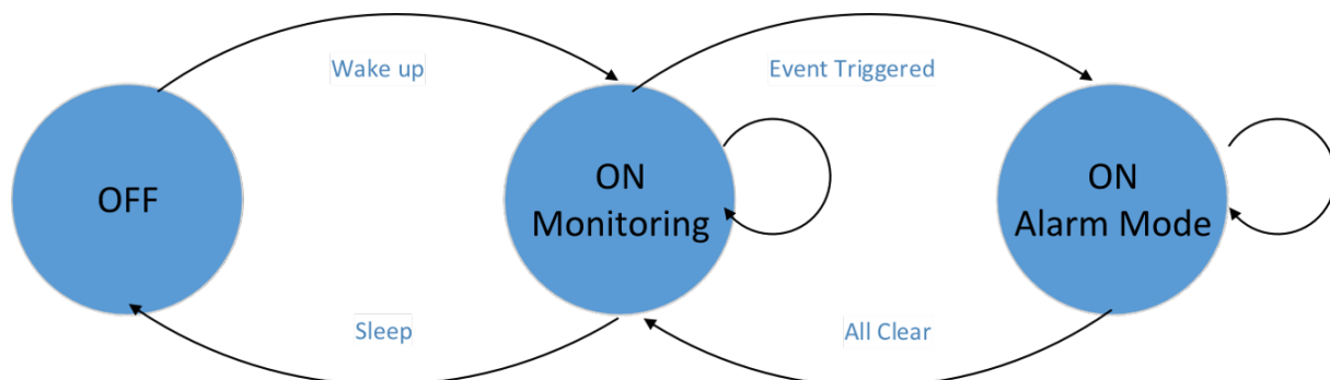
Figure 4-33: Traffic model
