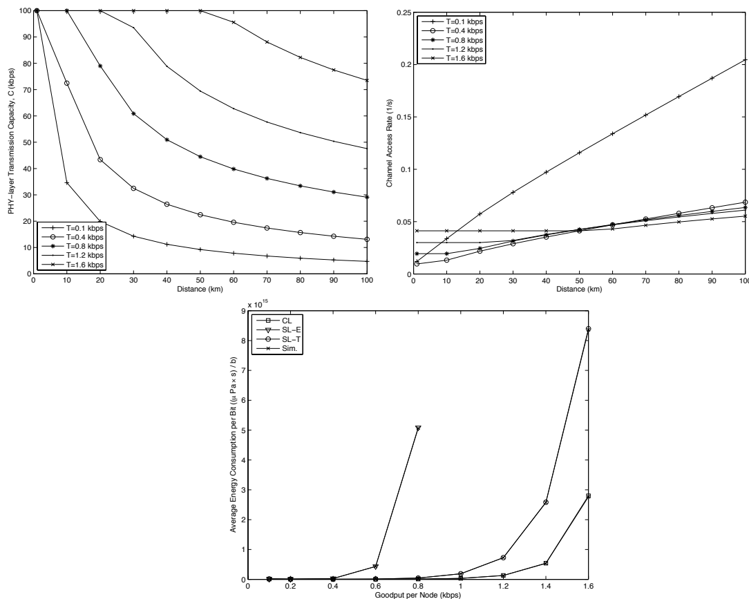
Figure 4-13: (a) Capacity allocations made by the proposed cross-layer policy (CL) (b) Channel access rate allocations made by CL. (c) Average energy consumption per bit for CL and SL policies as the goodput per node increases.
