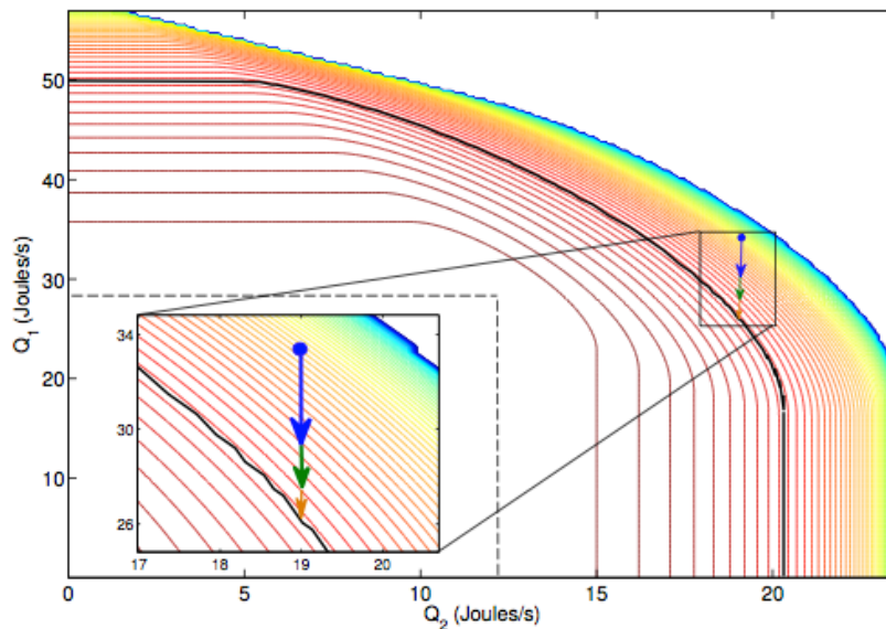
Figure 4-4: Performance of the proposed algorithm based on (4.1.9)
