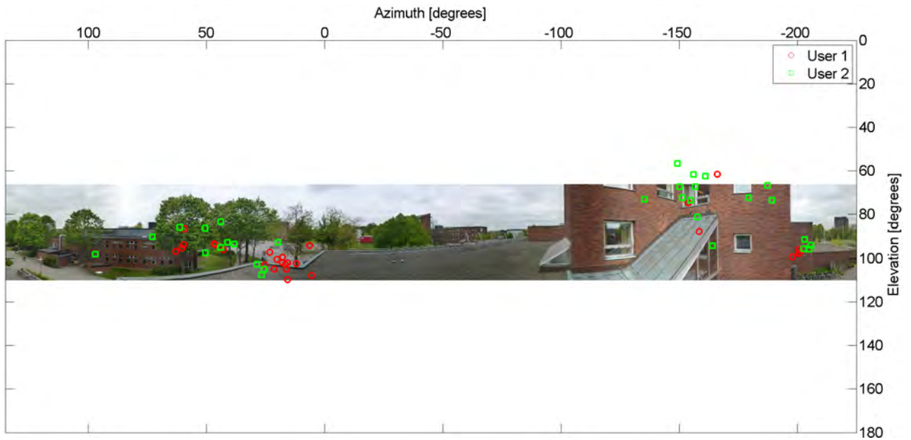
Figure 6.12: LOS component and the 30 strongest multipath components for users 1 and 2, at snapshot 100. This figure corresponds to an outdoor suburban microcell deployment (site MS 2). There is LOS to the BS and a crowd is present.
