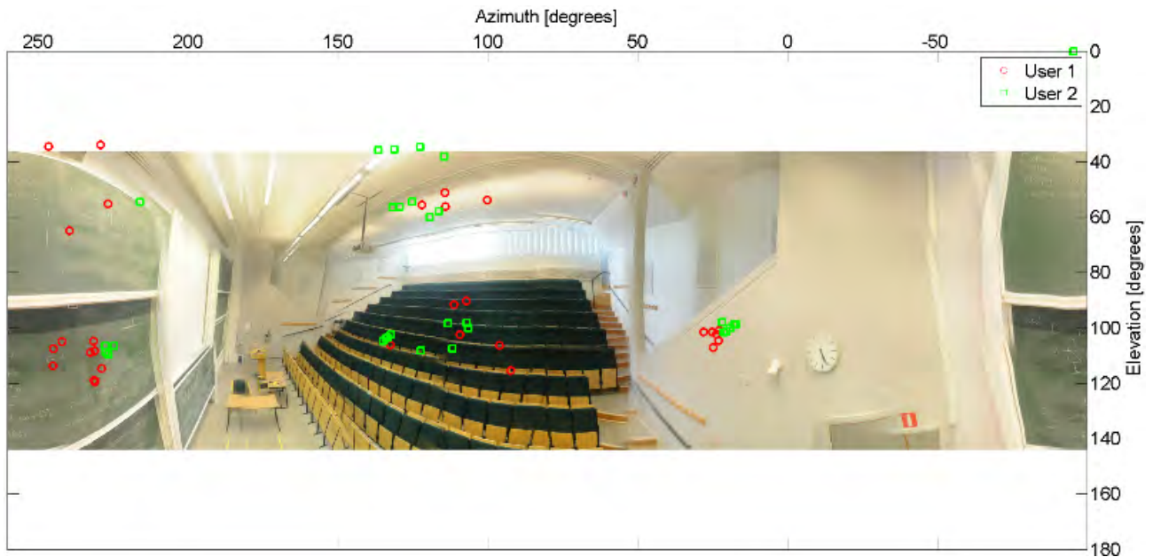
Figure 6.17: LOS component and the 30 strongest multipath components for users 1 and 2, at snapshot 10. This figure corresponds to an indoor auditorium deployment (BS 3, users at the center). There is LOS and no crowd is present.
