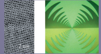
Fig.1. TEM image of the [001]-tilt \text{YBa}_2\text{Cu}_3\text{O}_{7-x} grain-boundary Josephson junction (left) and micrograph of the junction with integrated broadband antenna for Hilbert spectroscopy (right).
