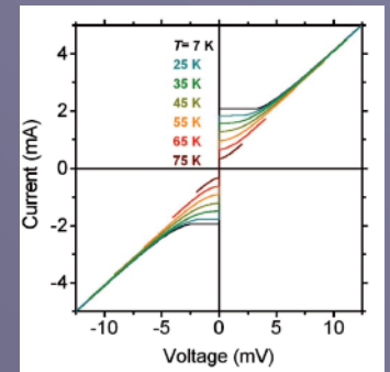
Fig.2. Current-voltage characteristics of the [100]-tilt \text{YBa}_2\text{Cu}_3\text{O}_{7-x} grain-boundary Josephson junction at various temperatures.
