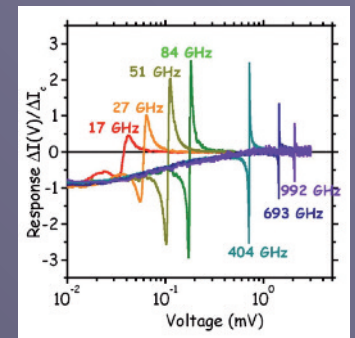
Fig. 3. Spectral range of the Hilbert spectroscopy using \text{YBa}_2\text{Cu}_3\text{O}_{7-x} grain-boundary Josephson junction at 85 K.
