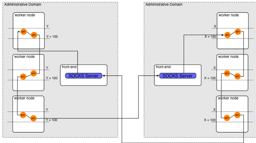
Figure 28: Operation of the Proxy technique.
