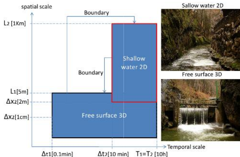
Figure 1: An example scale separation map (in this case of the irrigation canal application).
