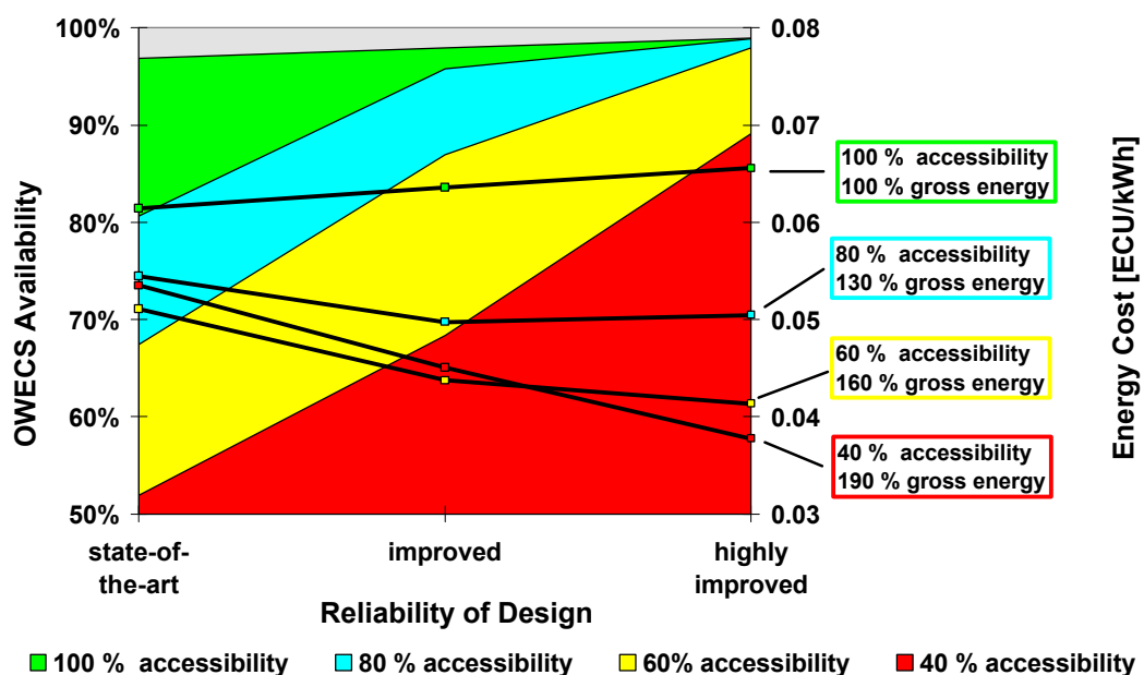
Figure 2.16: Availability vs. improved reliability
