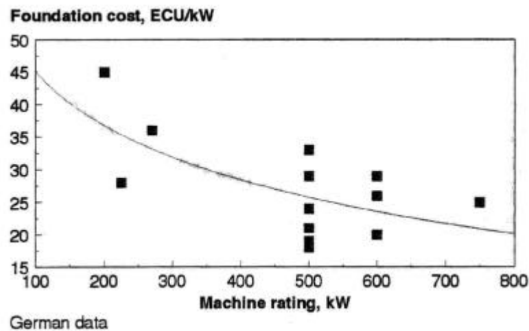
Figure 2.15 Foundation cost v rated power
