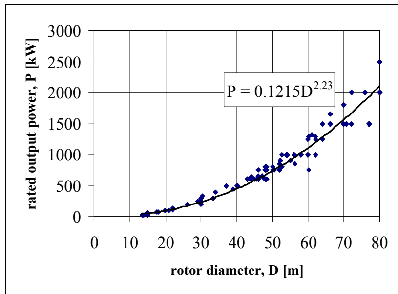
Figure 2.2 Power rating of wind turbines
