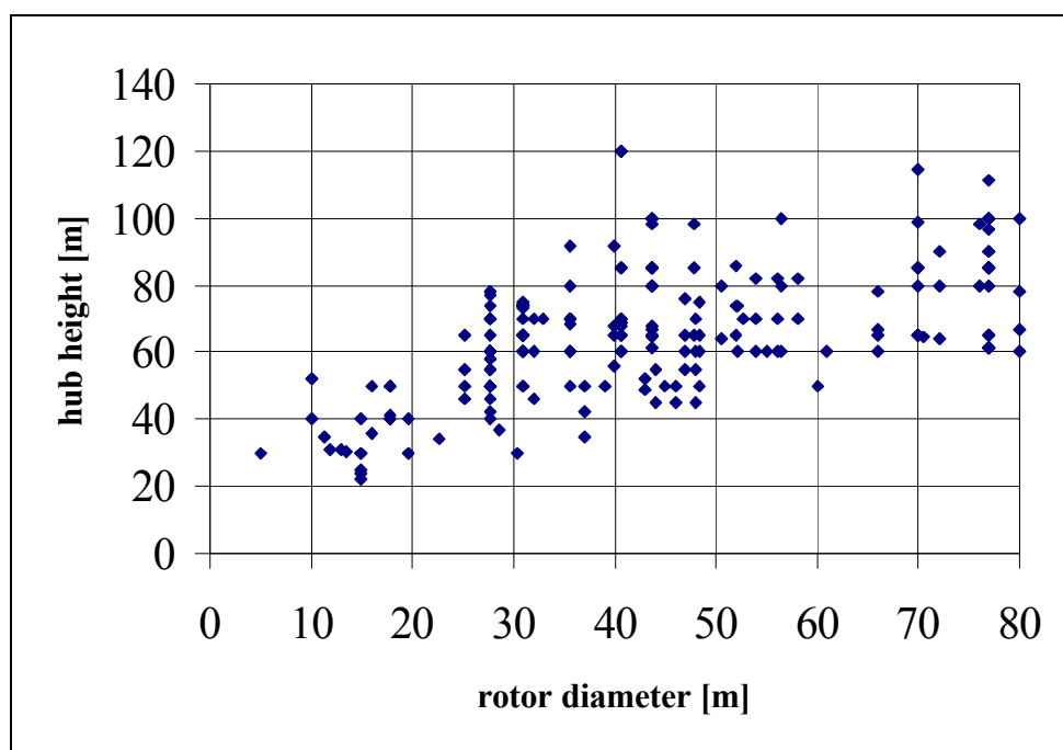
Figure 2.4 Hub height variation of wind turbines
