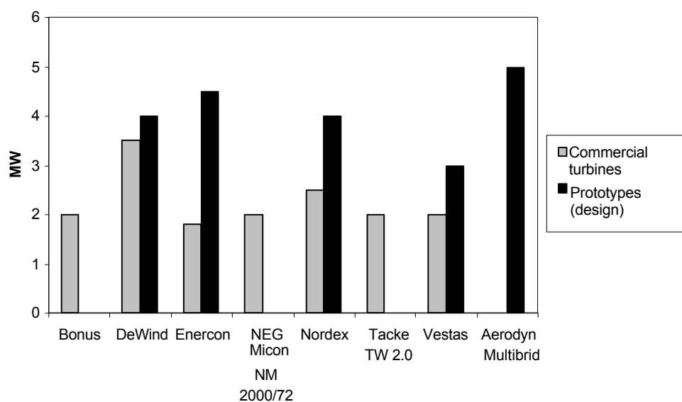
Figure 2.6 Commercial offshore turbines and forthcoming prototypes
