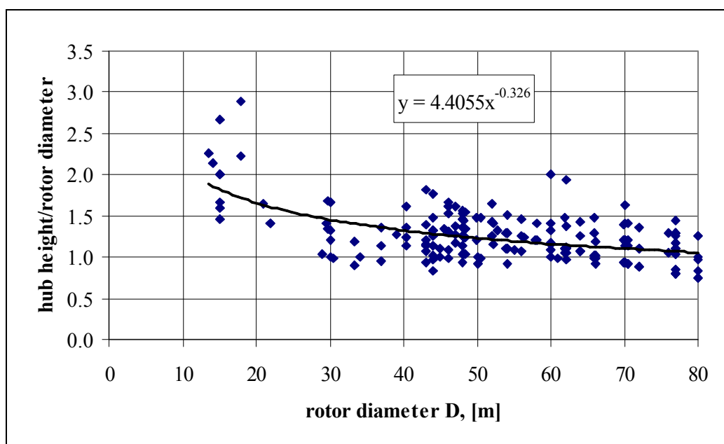
Figure 2.10 Hub height/rotor diameter ratio
