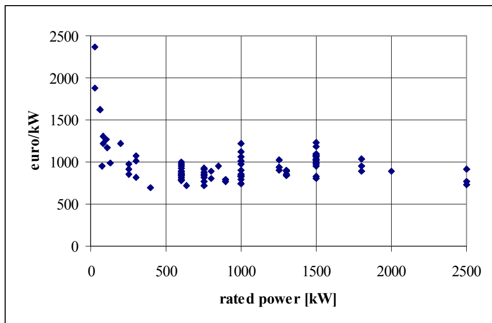
Figure 2.14 Cost per kW v rated power
