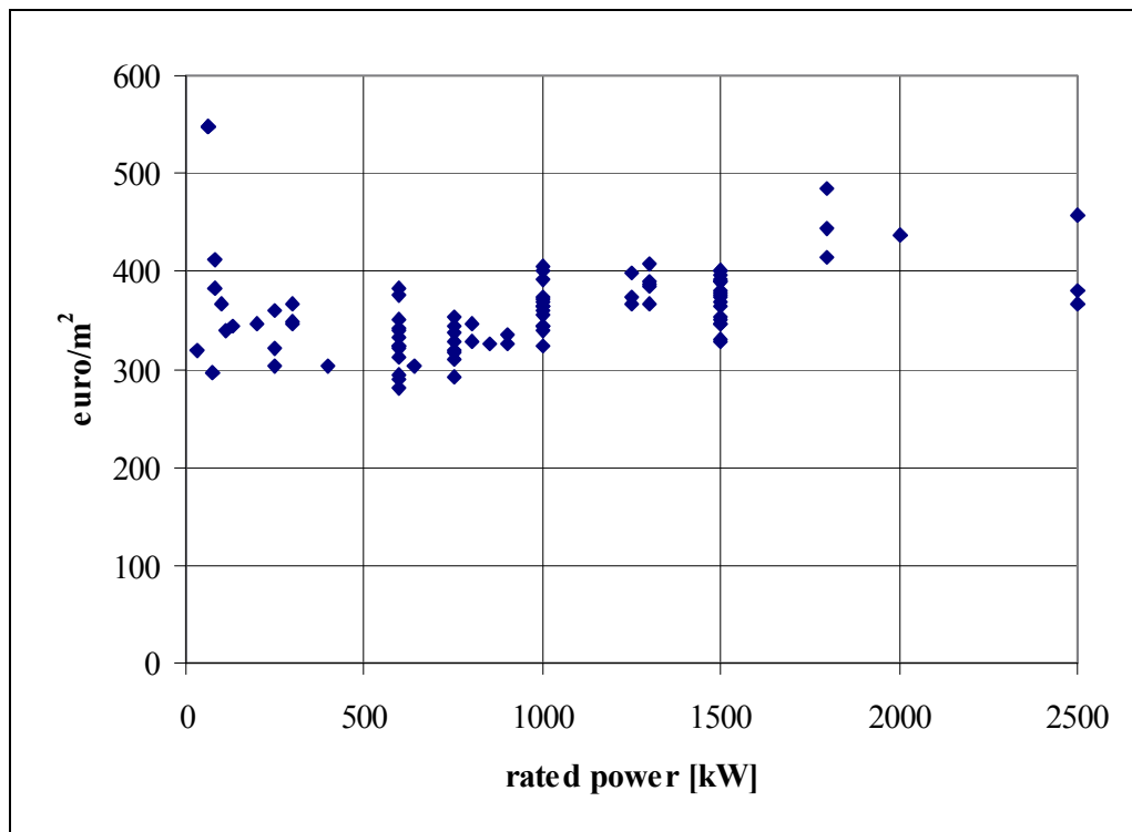
Figure 2.13 Cost per unit swept area v rated power
