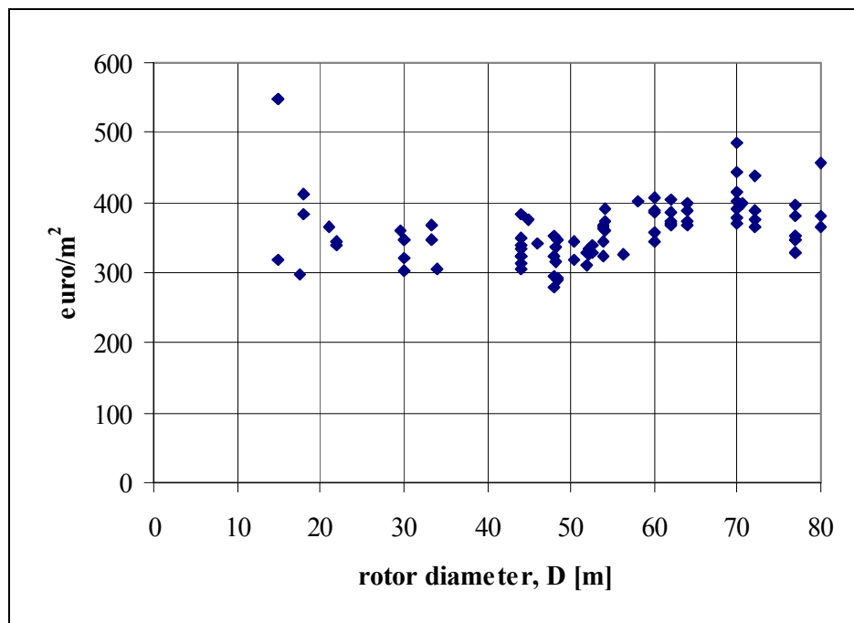
Figure 2.12 Cost per unit swept area v diameter
