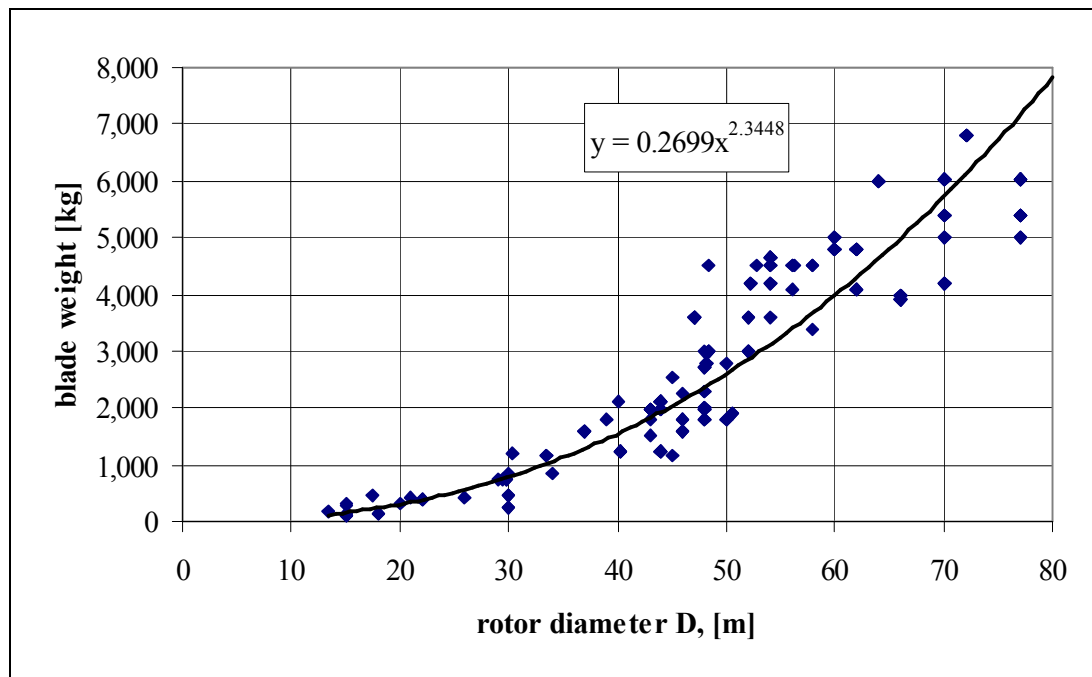
Figure 2.7 Blade mass related to rotor diameter
