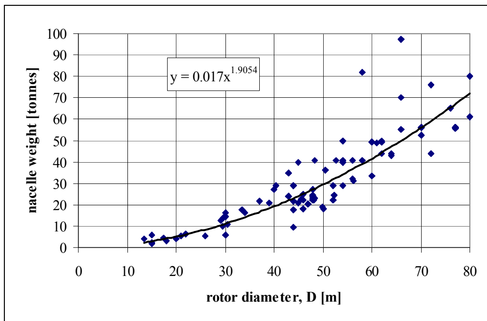
Figure 2.8 Nacelle mass v rotor diameter
