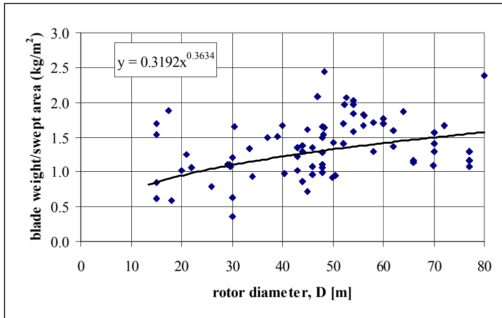
Figure 2.9 Rotor mass/ swept area ratio
