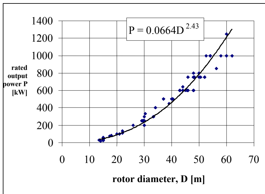
Figure 2.1 Power rating of wind turbines up to 62 m diameter
