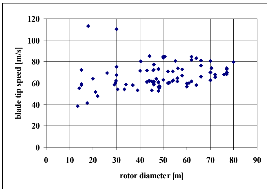
Figure 2.3 Design tip speed (maximum steady state)
