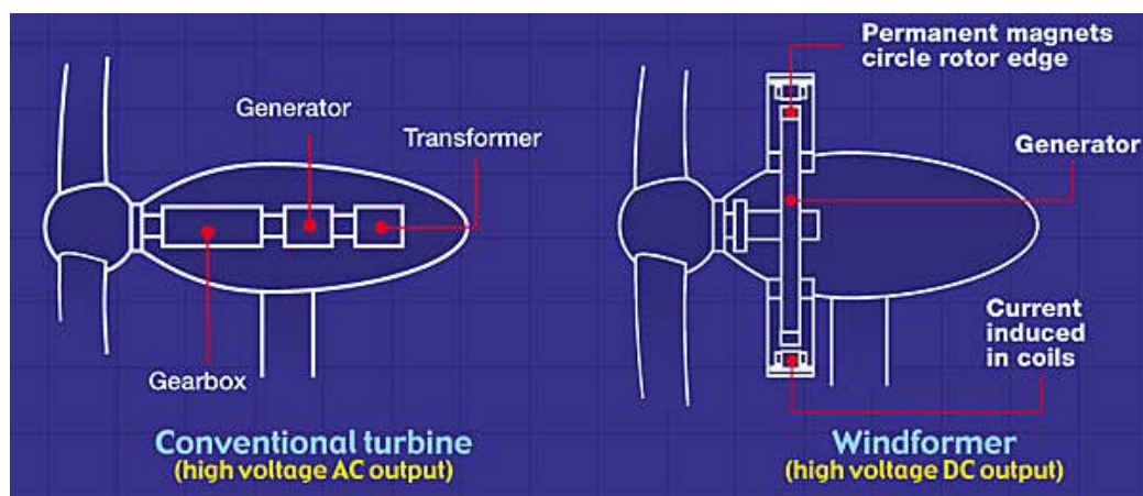
Figure 2.18 Diagram comparing conventional and Scanwind concepts (Source http://www.newscientist.com/news/news_224335.html )
