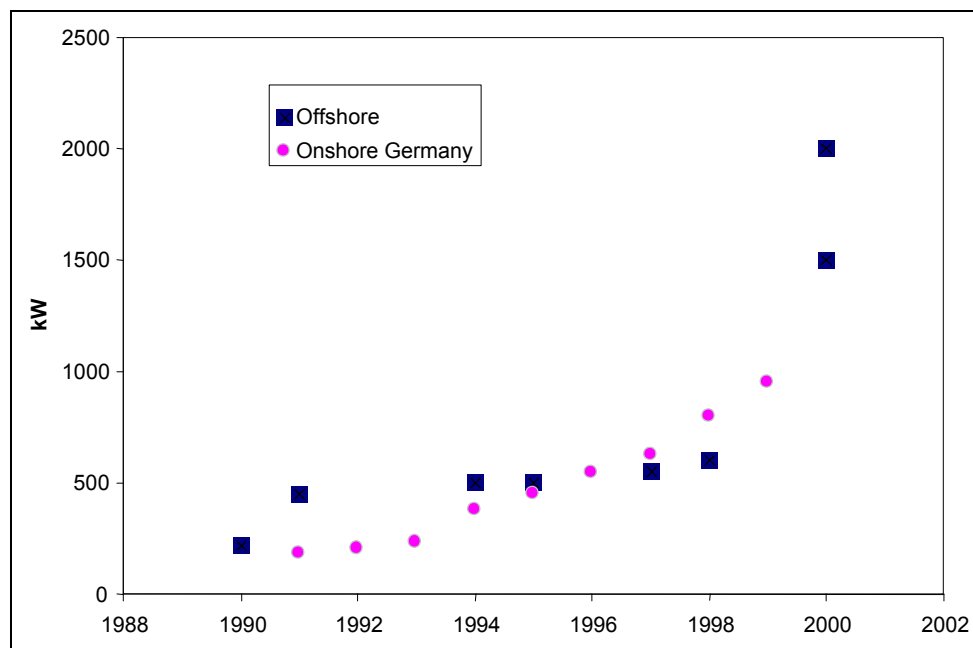
Figure 2.5 Rating trends in land based and offshore wind turbines
