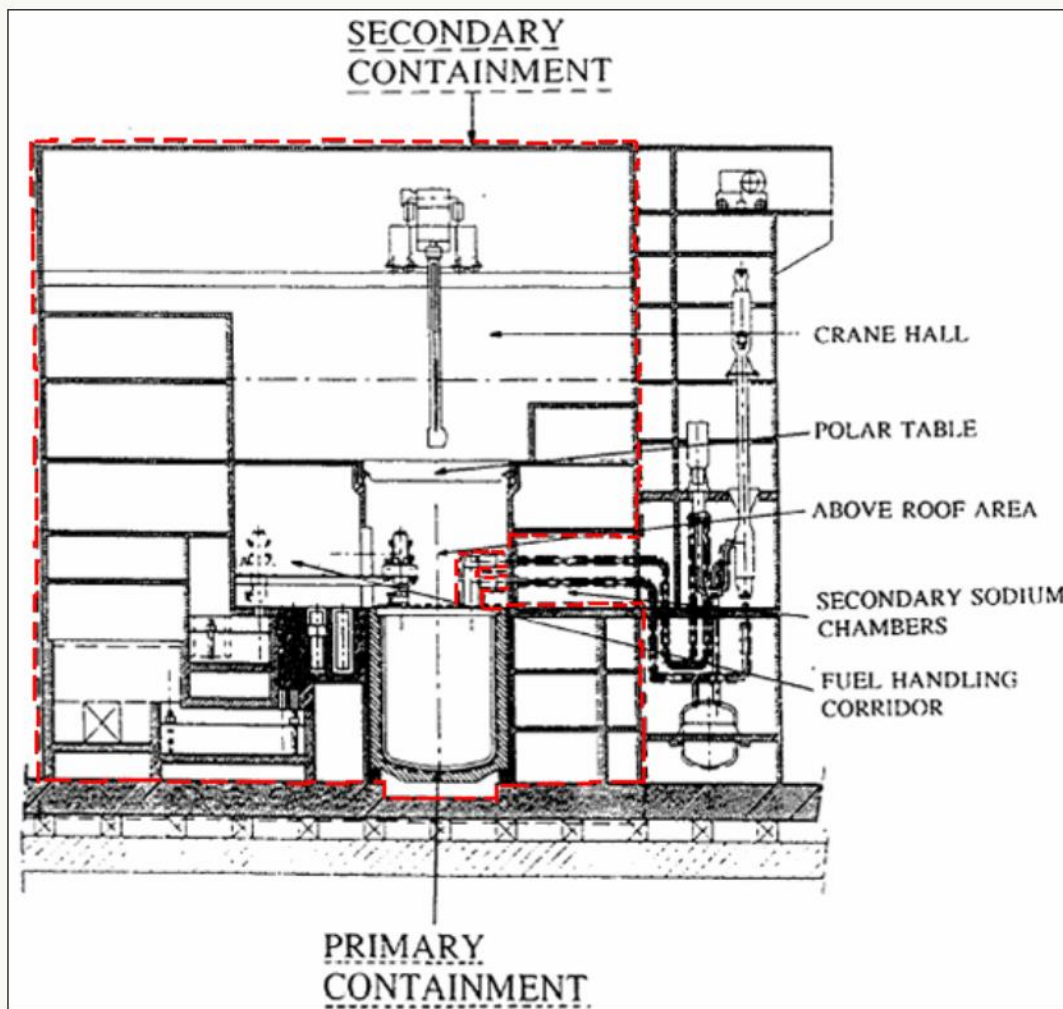
Figure 12: EFR - Secondary containment boundary
