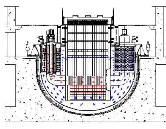
Figure 9 : sketch of ELSY primary circuit
