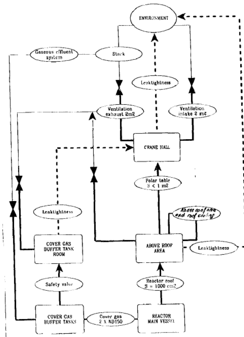
Figure 13: EFR - Release ways of radiological products
