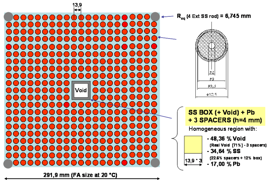
Figure 4: Schematic view of the square fuel rod lattice
