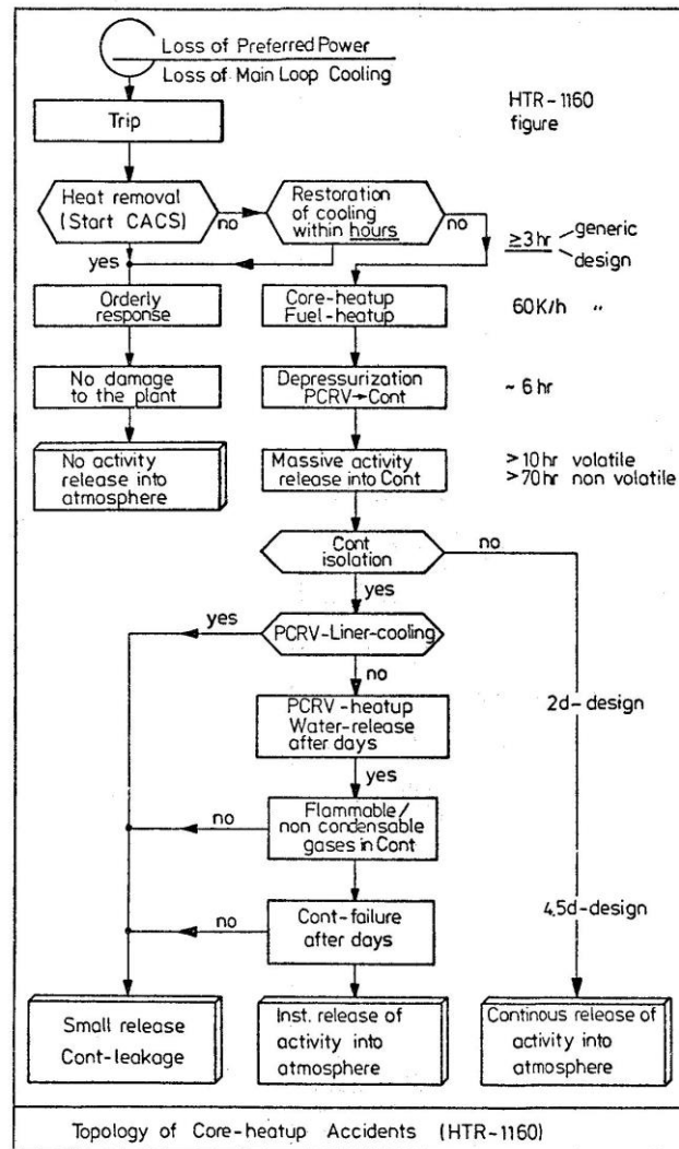
Figure 18: Topology of FP release during core heat-up accidents in VHTRs
