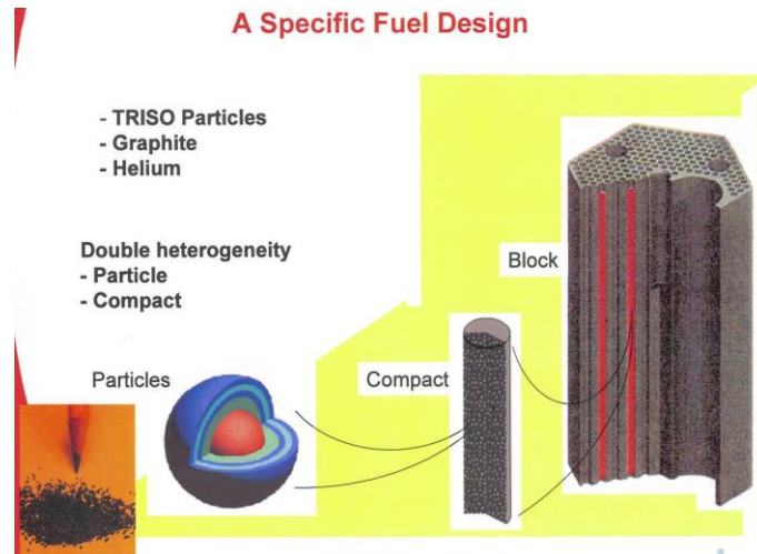
Figure 6: prismatic blocks for VHTR (ANTARES)
