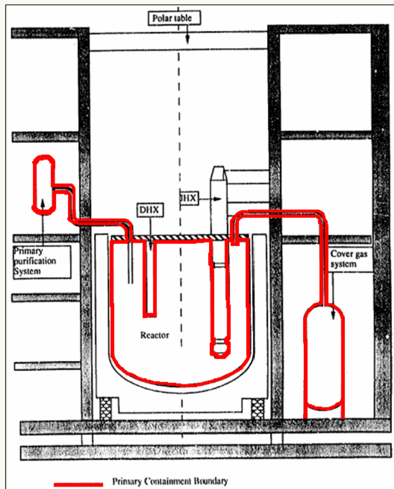
Figure 11: EFR - primary containment boundary
