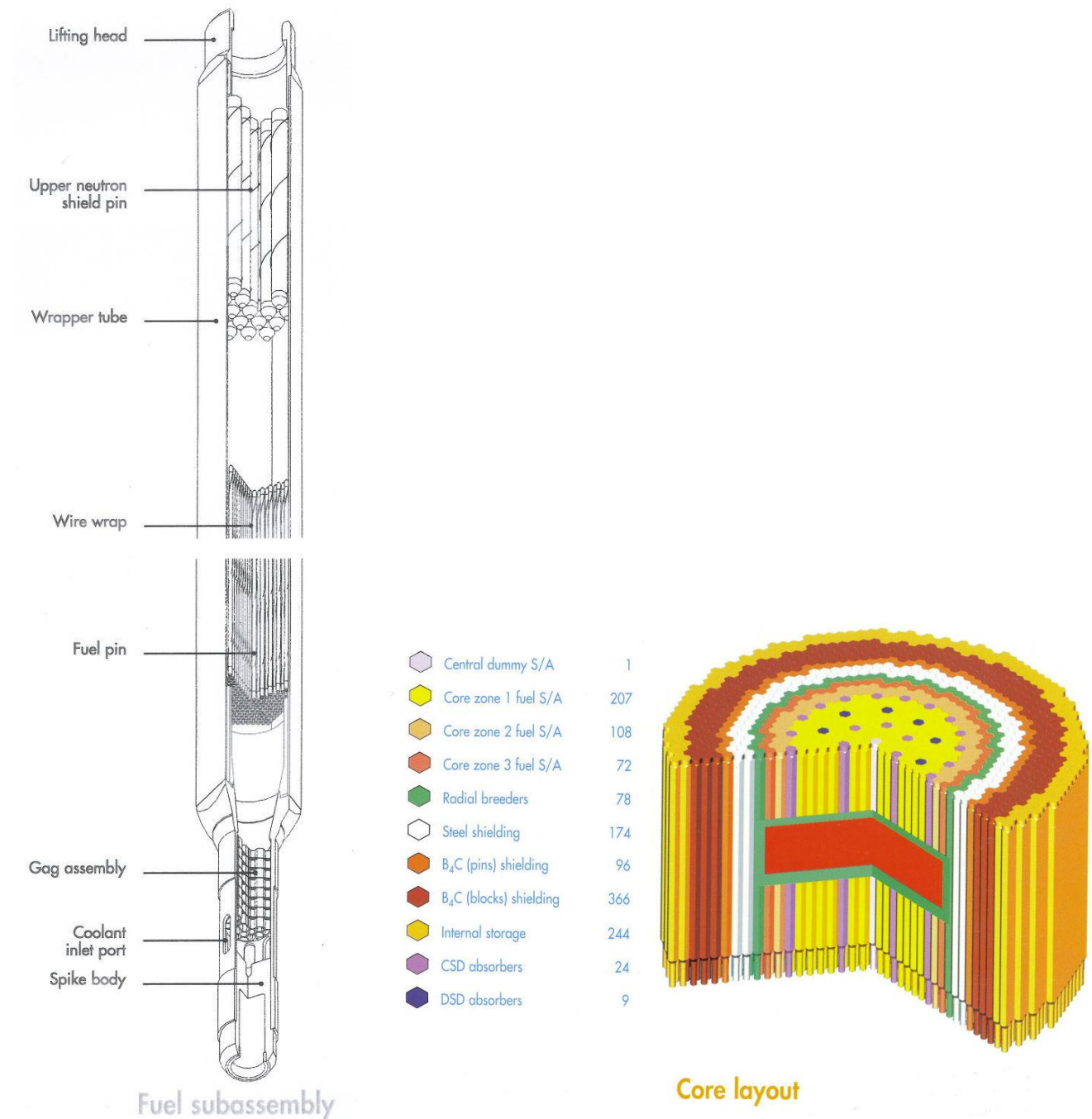
Figure 2: EFR pin fuel and core arrangement
