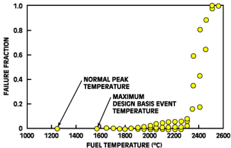
Figure 16: Integrity of MHTGR coated fuel particles as function of temperature [ref VHTR-2.3.1_2]
