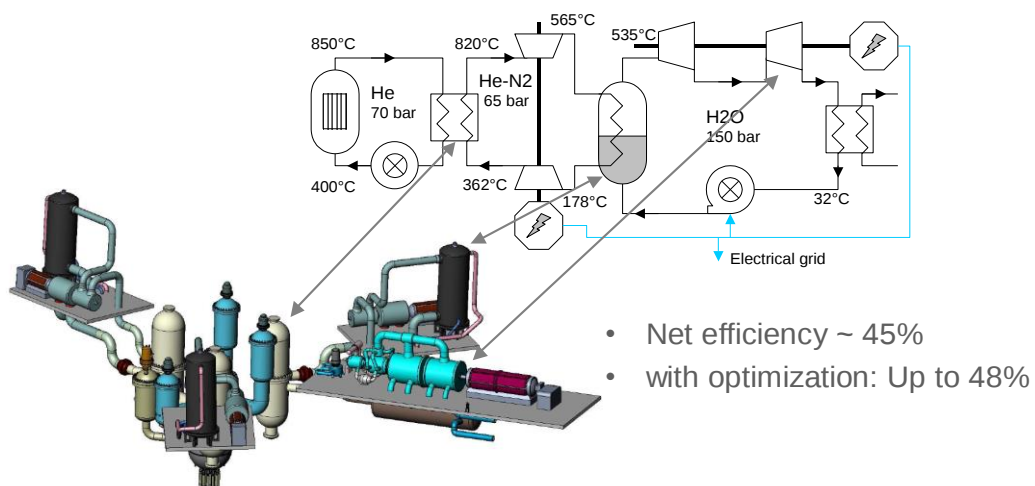
Figure 8: Layout of the GFR normal loops featuring a combined Brayton cycle
