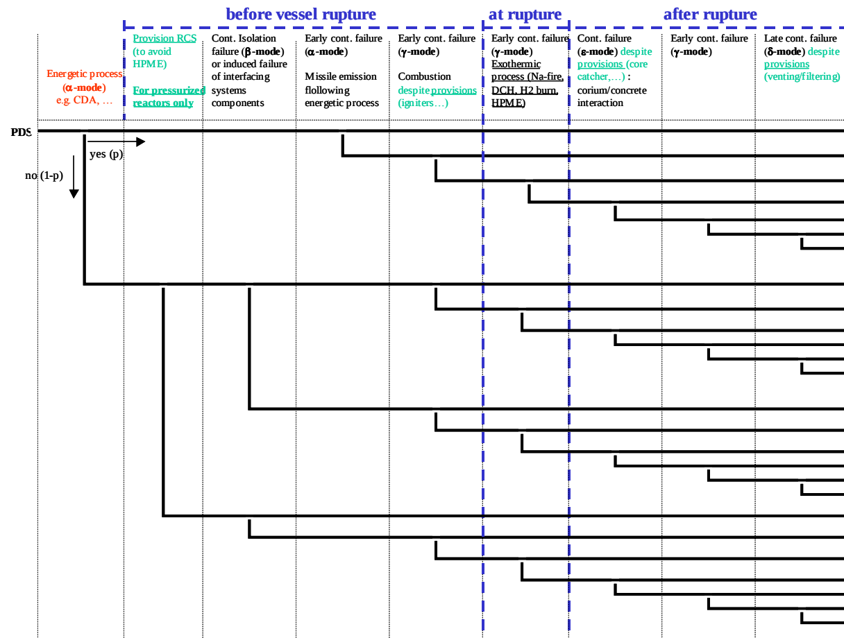
Figure 19: Generic Event Tree related to containment degradation modes
