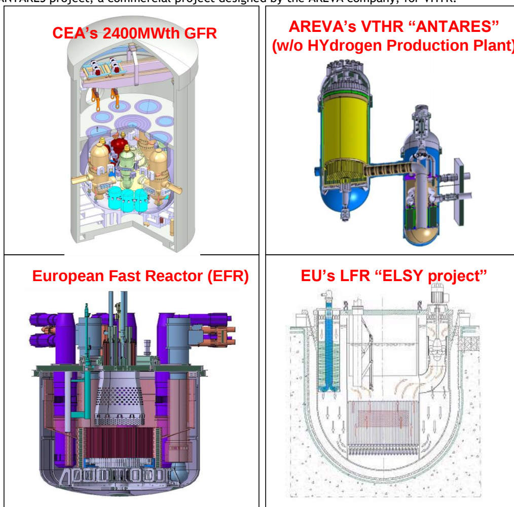
Figure 1: Overview of the four “representative” Generation IV concepts
