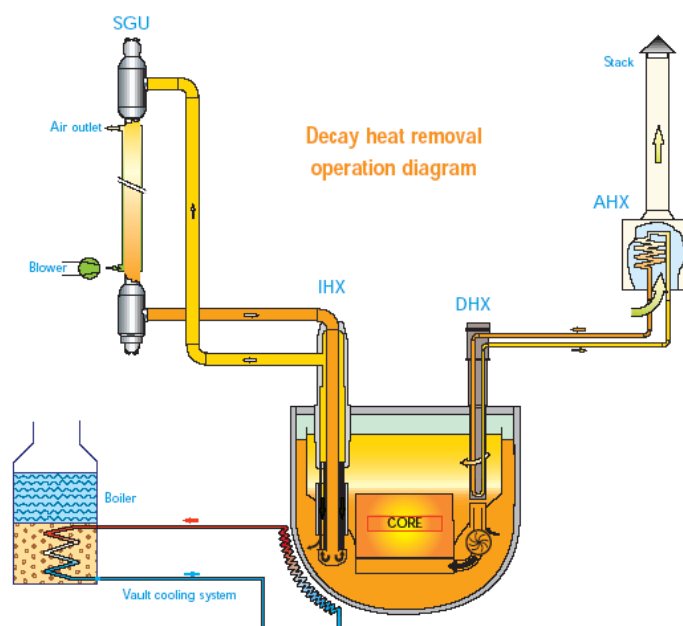
Figure 7: EFR 98 - DHR systems
