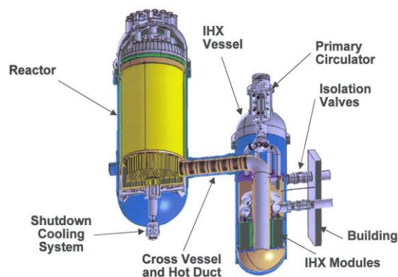
Figure 10: sketch of ANTARES primary circuit
