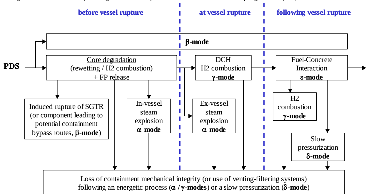
Figure 15: Flowchart of the containment degradation modes with the time frame of the severe accident progression
