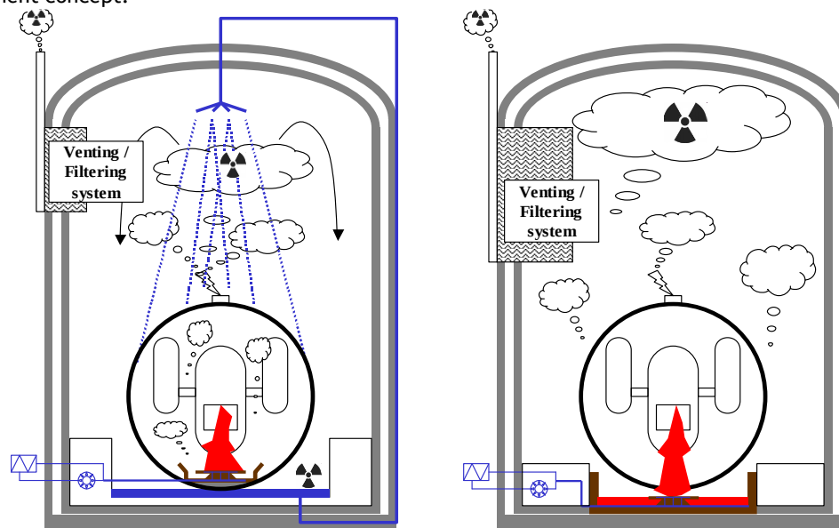
Figure 17: tentative sketches of GFR containment features for FP retention enhancement
