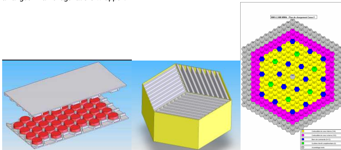
Figure 3: GFR plate-type fuel and core arrangement
