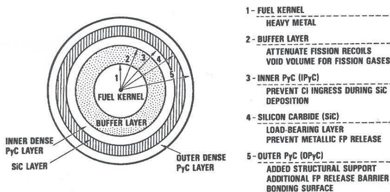
Figure 5: TRISO particles for VHTR
