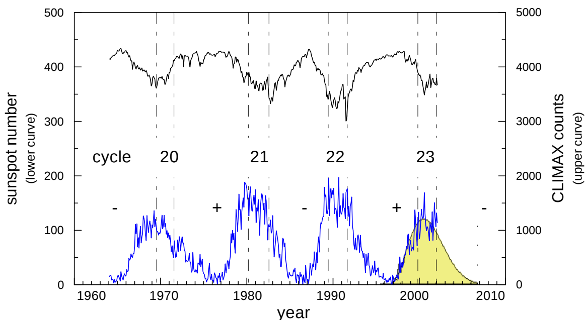
Figure 4.1 Sunspot number (lower curve) and monthly averaged Climax neutron monitor count rate per hour (divided by 100) for solar cycles 20 through 23 (from 1964 to begin of 2002). Solar cycle 23 is expected to last until approximately the year 2008. The vertical dashed lines indicate the periods (around 2 years each) of solar reversal; +/- specifies the respective polarity of the field model of NASA Johnson Space Center. The shaded area is the solar activity predicted by the NASA Marshall Space Flight Center.
