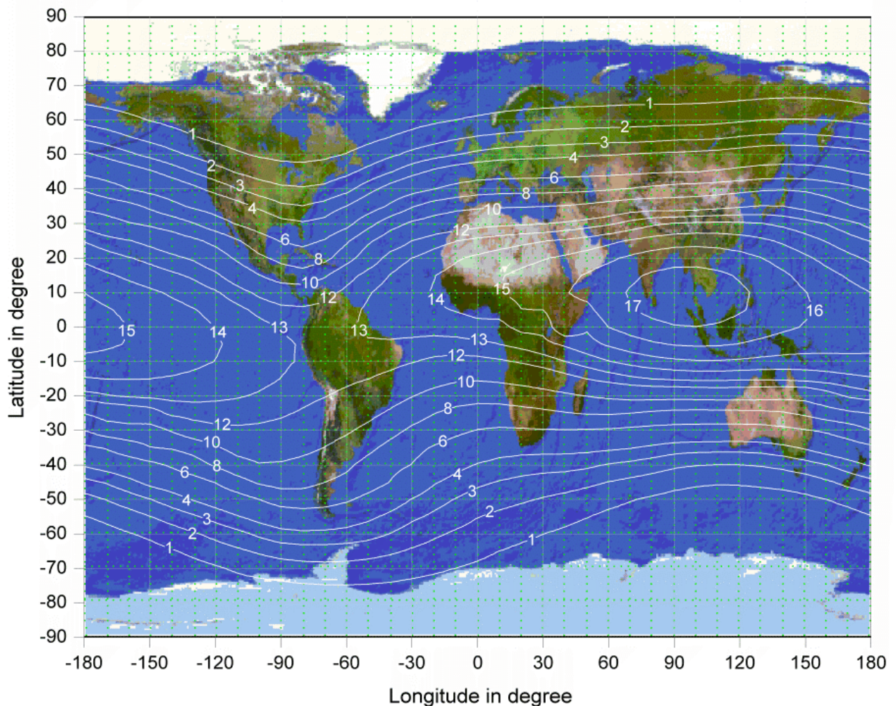
Figure 4.4 Vertical Cosmic Ray Cut-off Rigidity in GV based on data in 1990 at 20 km altitude.
