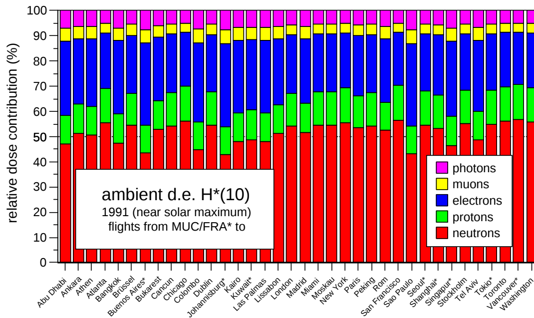
Figure 4.3 Relative contribution to ambient dose equivalent, H^*(10) , for various destinations near solar maximum condition (1991) for 37000 ft flight altitude, as calculated with EPCARDv3.2. Data are shown in alphabetic order.
