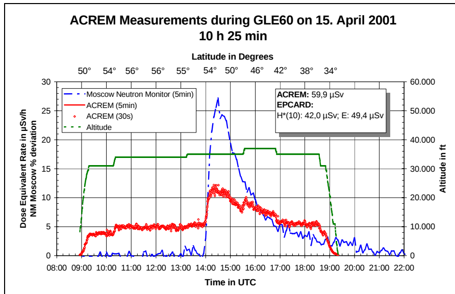
Figure 4.6. Measurement results during GLE 60. The dose measurement results (red) starts to increase at the same time as the neutron monitor (blue) at ground. Flight altitude is marked with green.
