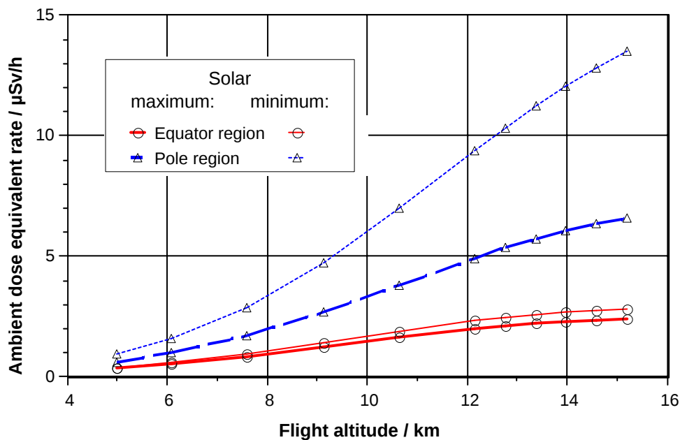
Figure 4.2 Calculated ambient dose equivalent rate, dH^*(10)/dt , for conditions close to solar maximum activity in Jan.1990 thick lines and close to solar minimum in Jan. 1998 thin lines, both at zero-meridian ( \lambda=0^\circ ) and geographic latitude \phi of 0^\circ (red lines) resp. 90^\circ (blue lines).
