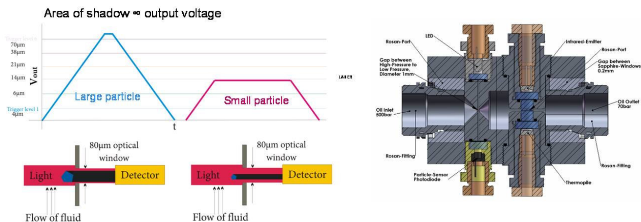
WP 2 - Figure 4 - Particle sensors developed by EADS-IW-D.
