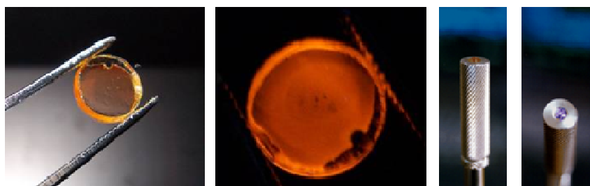
WP 2 - Figure 2 - Orange-luminescent sensor films developed at UCM to monitor chemical species in hydraulic fluids. The polymer film (20–30 µm) is chemically attached to a 9-mm glass disk. The stimuli-sensitive window is then mounted inside a stainless steel encasing.
