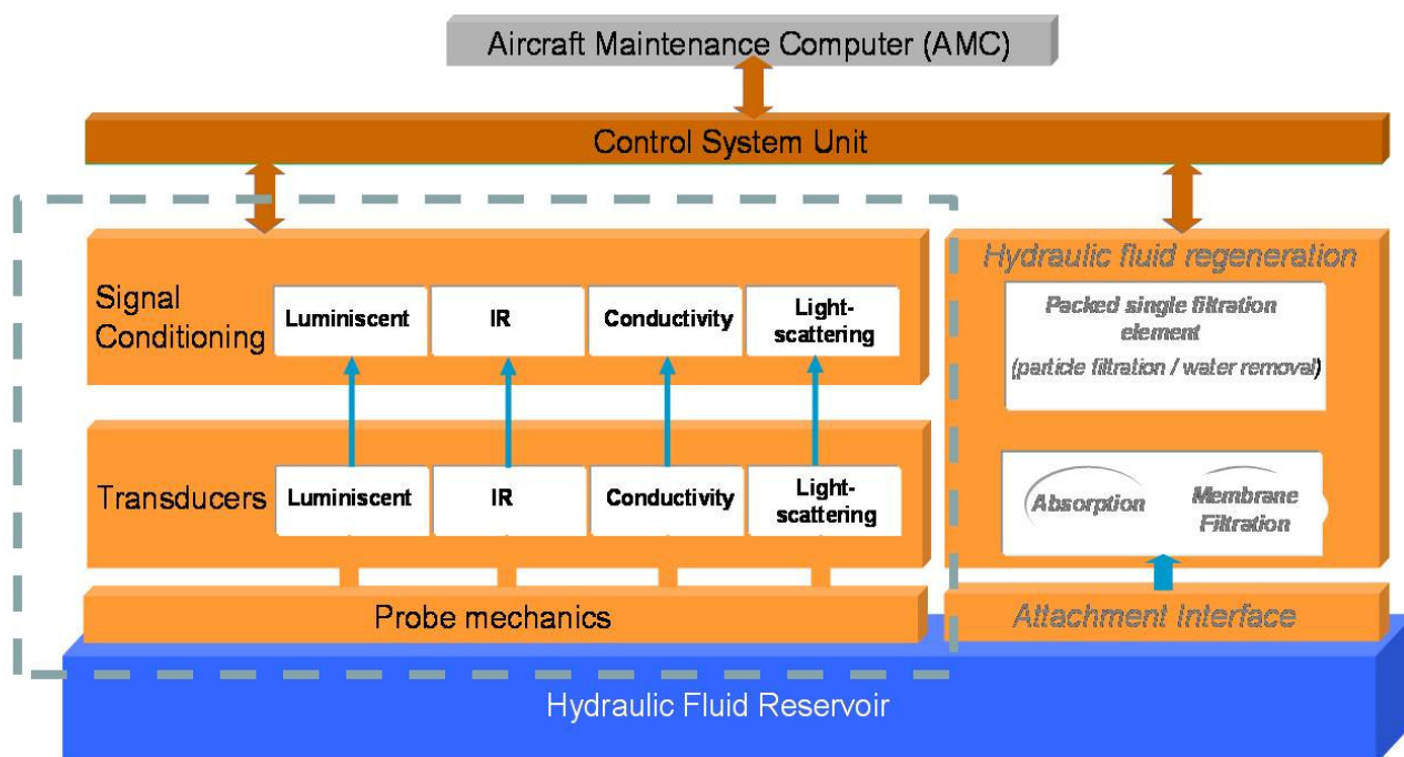
Figure 2 - SuperSkySense system block diagram
