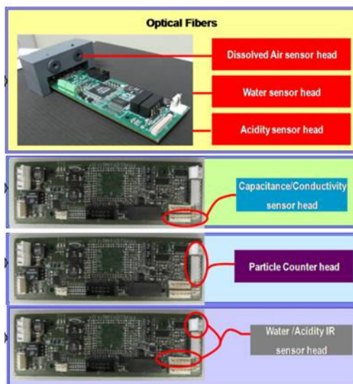
WP4 - Figure 2 - SSK Sensor electronics
