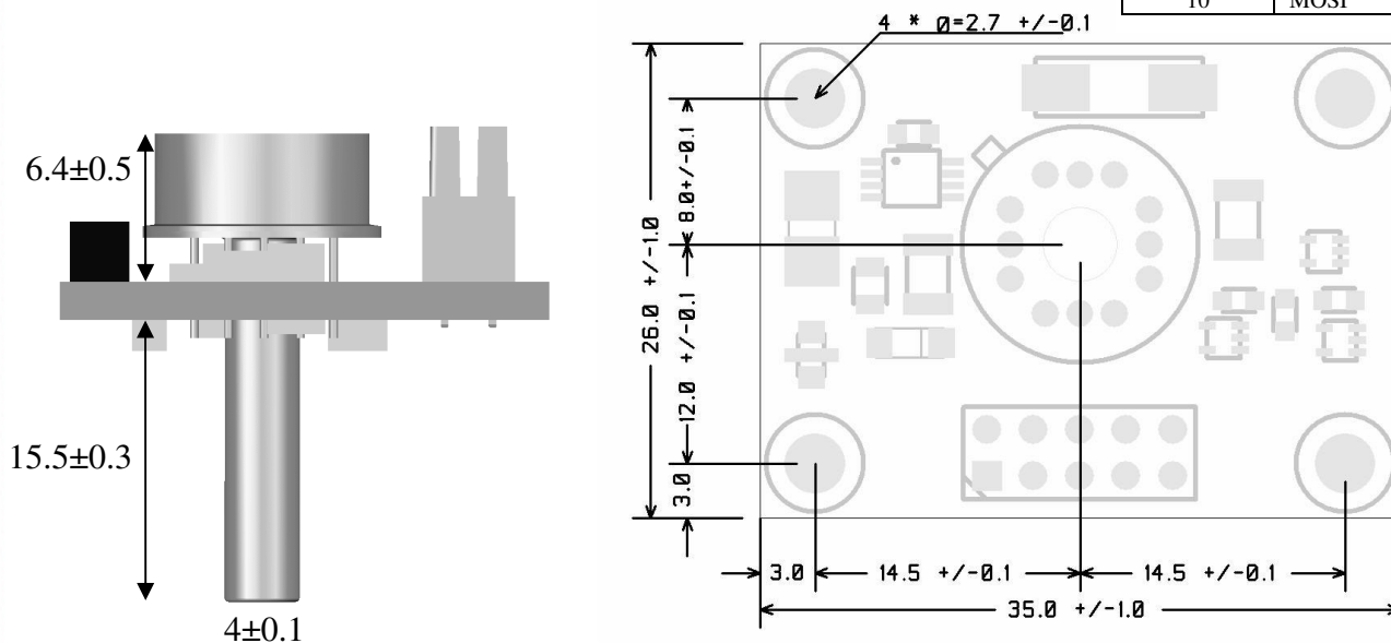
Figure 1 – Mechanical dimensions in mm
