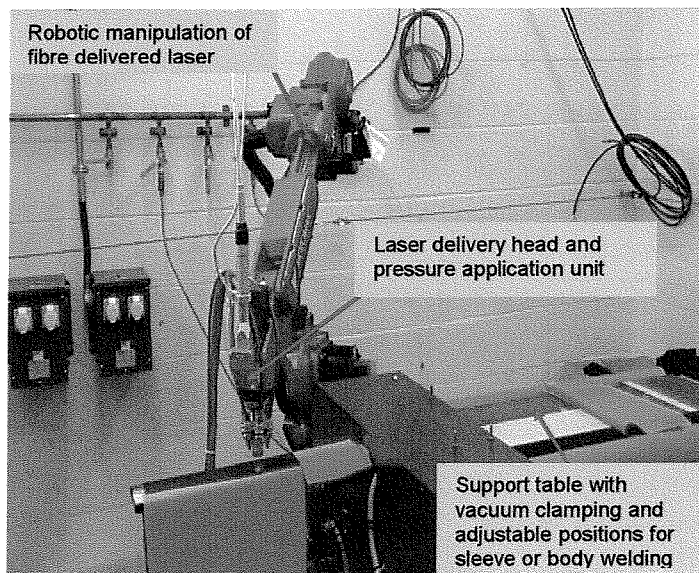
Fig.3 Automated laser welding equipment.
