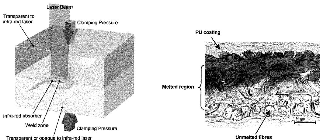
Fig.2 Laser welding uses transmission of energy to weld without melting the outer surfaces.
