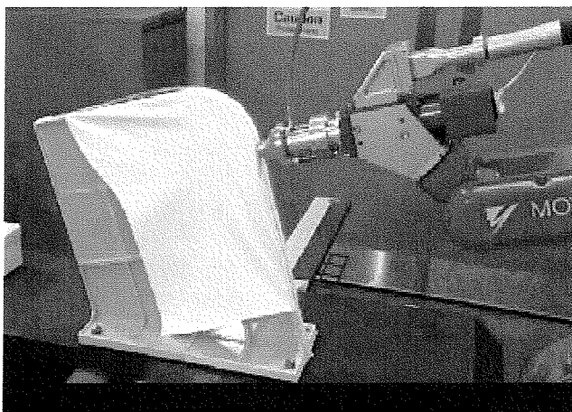
Fig.5 3D processing for a hood seam
