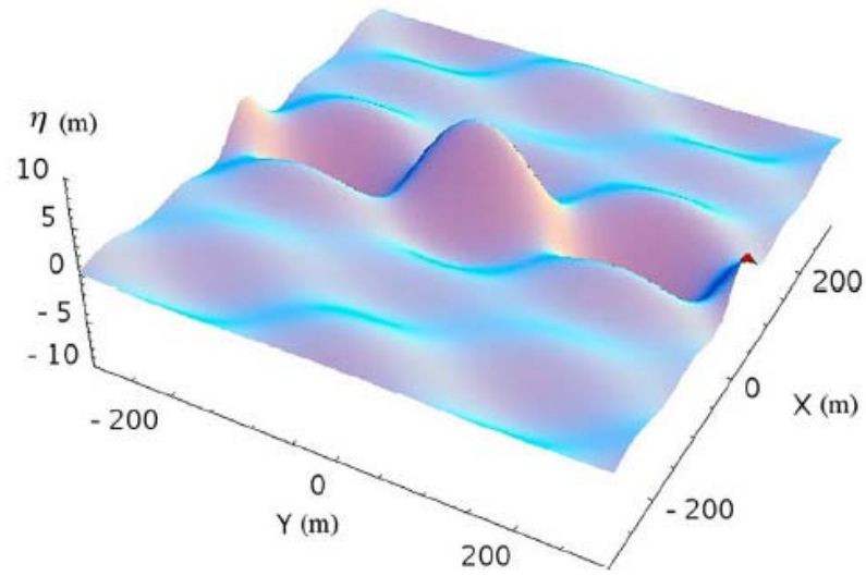
Figure 1. The surface elevation corresponding to the breather solution with the angle b between the two wave systems equal to 50 degree.
