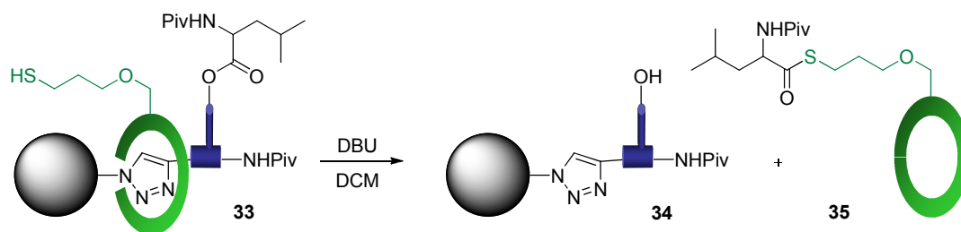
Scheme 3. Operation of a test model peptide synthesizer with a single amino acid residue.
