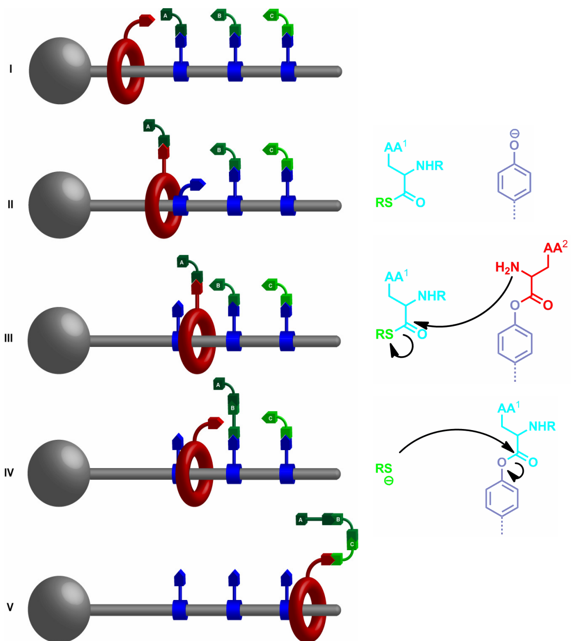
Scheme A cartoon depiction of a rotaxane-based molecular machine capable of sequence specific peptide synthesis.
