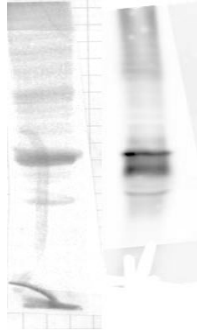
Fig. 1. IRT1 purification. Coomassie blue staining of enriched IRT1 fraction resulting from Ni-affinity chromatography (left). Immunoblot of the same fraction using anti-IRT1 antibody (right)
