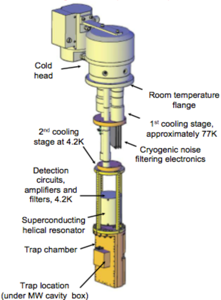
Drawing of the inner experimental setup
