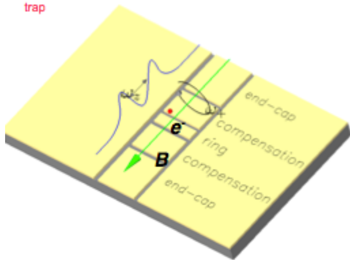
Sketch of a basic Coplanar Waveguide planar Penning trap
