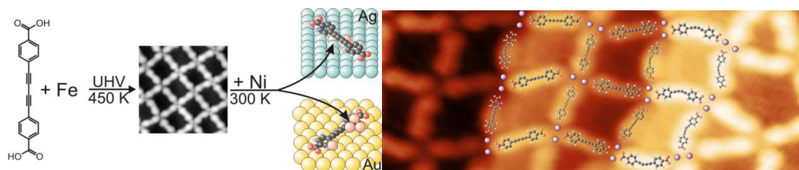
Figure 1: The basic concept of experimental study on adaptive coordination networks – formation of metal-organic template and its hierarchical decoration by Ni atoms (left) and representative STM image of highly adaptive metal-organic coordination network on Au(111) surface (right).
