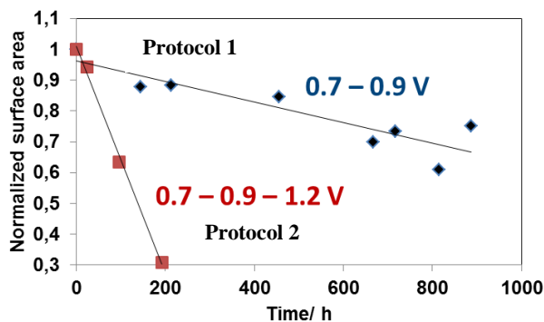
Figure 4: Normalized active cathode catalyst surface area measured during AST, SC1.
