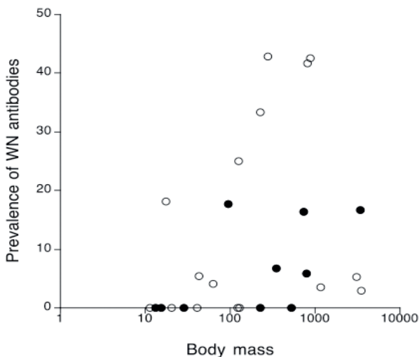
Figure 1. Prevalence of WNV neutralizing antibodies in different avian species. The prevalence of antibodies was higher in migratory species (open circles) than in resident species (filled circles). Antibody prevalence also increased with the body mass of species. (Based on the dataset analysed by Figuerola et al. 2008).
