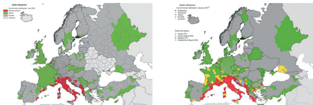
Figure 6. Distribution maps of invasive mosquito species Aedes albopictus in Europe in June 2010 (left) and January 2015 (right)
