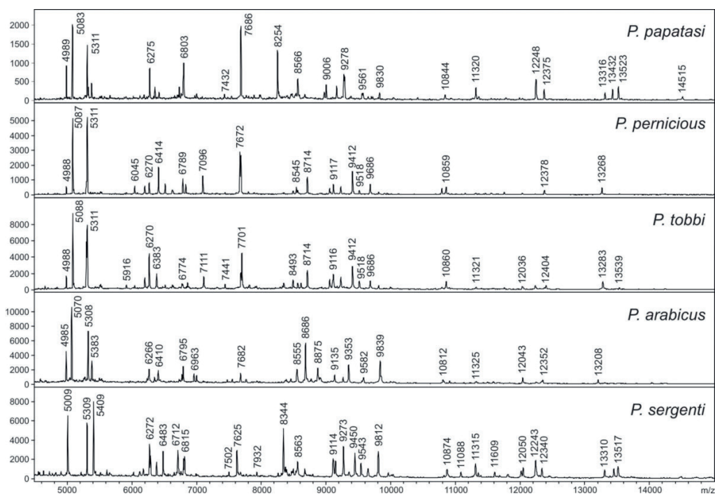
MALDI-TOF MS protein profiles of five different species of the genus Phlebotomus showing species-unique peaks for conclusive species identification. The peaks in the mass spectra represent peptides or small proteins obtained from the sand fly bodies using acidic extraction.
