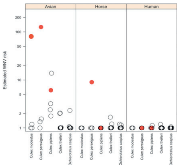
Figure 2. Estimated risk of WNV transmission by different mosquito species in different localities. Transmission risk is calculated as the product of vector abundance, vector competence, fraction of mosquito females feeding on competent hosts (birds) and the fraction of mosquito females feeding in the group of interest (birds, horses or humans). Filled circles indicate the cases where WNV has been detected in the mosquito pools. The figure has been redrawn from Muñoz et al. (2012) original data, updated with new virus detection information and the risk values calculated considering that chickens are not competent hosts for WNV.
