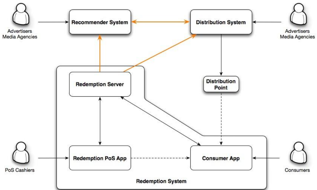
Figure 1: The Dicore2s System Overview
