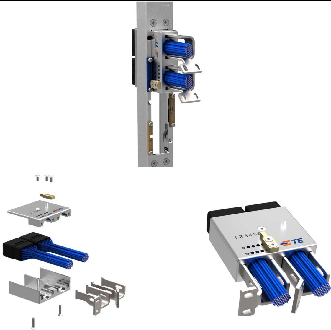
Picture 24 : TYCO - Direct aircraft connection (cabinet side)
