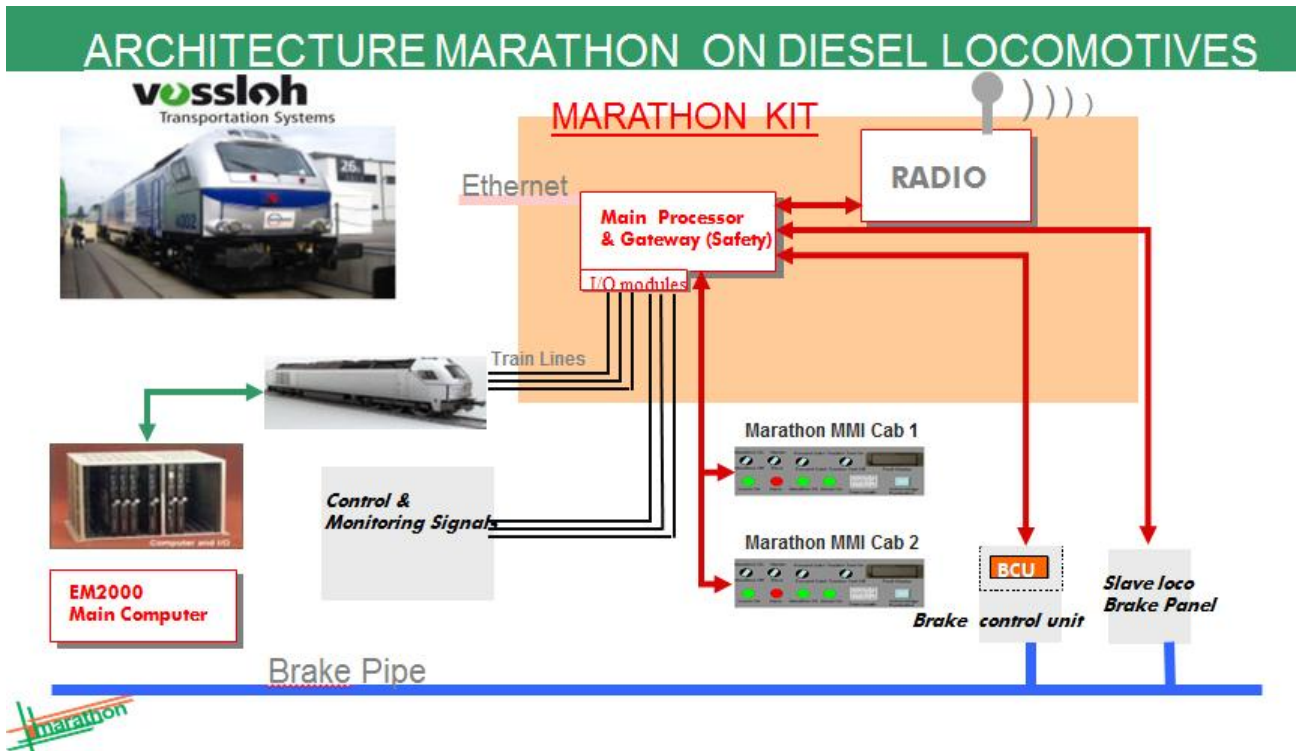
Figure 2 – MARATHON Architecture on Diesel Locomotives
