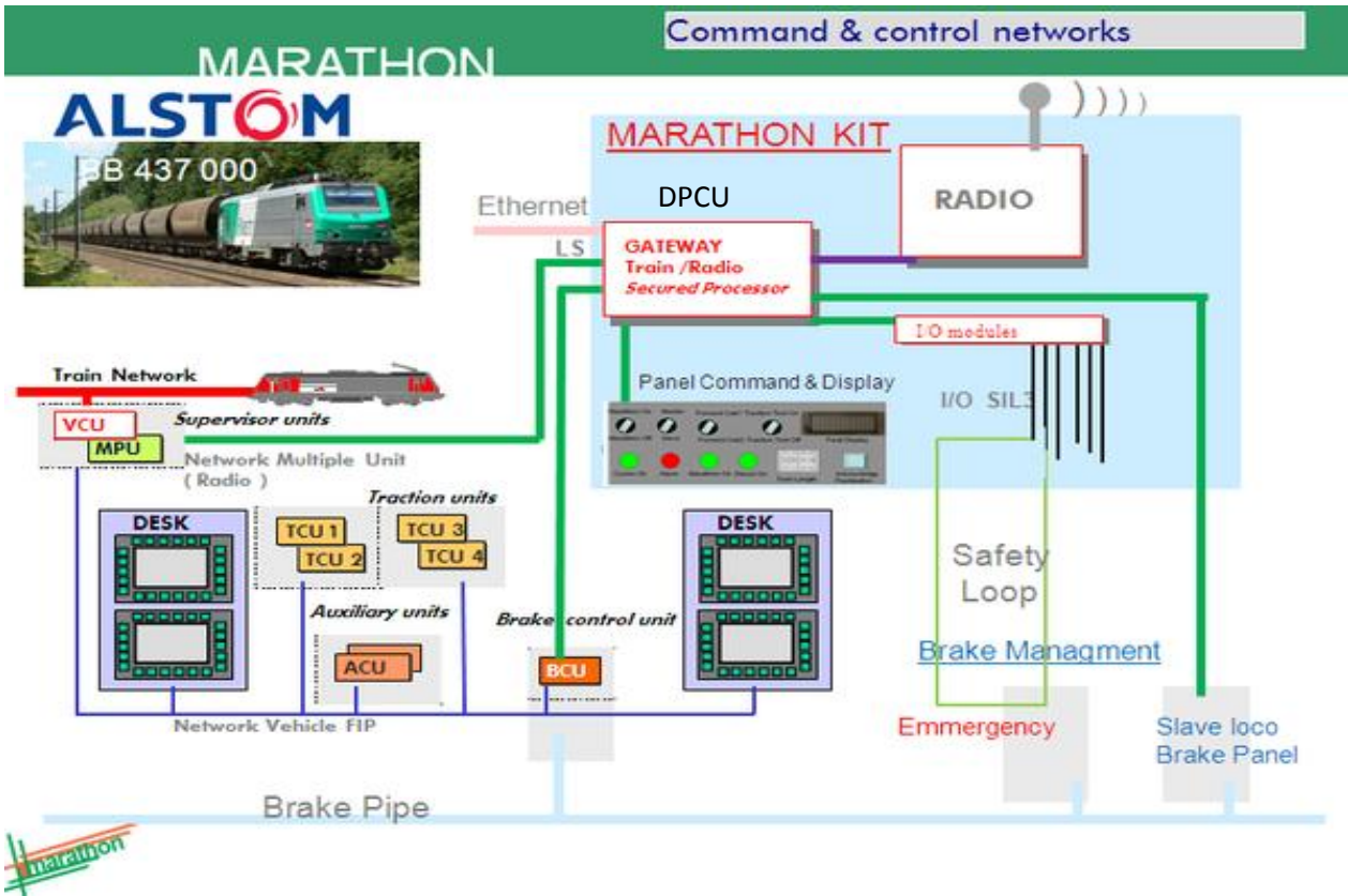
Figure 3 – MARATHON Architecture on BB 437000 Locomotives
