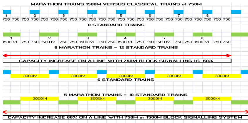
Figure 6 – MARATHON – Capacity Results
