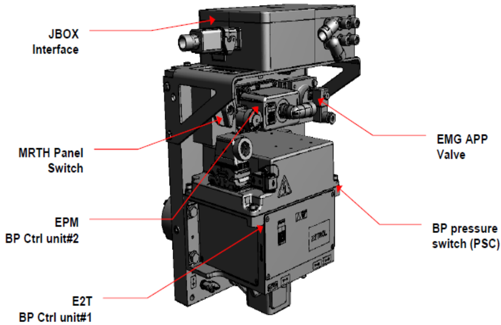
Figure 1 – Brake Slave Unit
