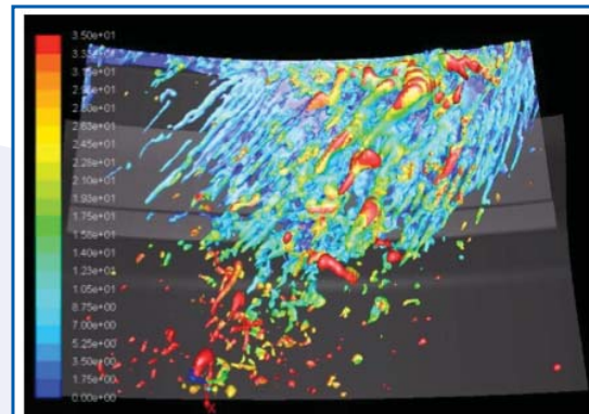
VoF LES of fuel film
