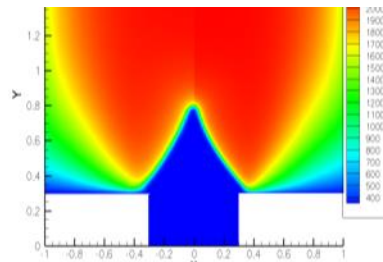
Figure 53: Temperature result using Lamfla2D (TUE, van Oijen), left and PRECISE-UNS using the DLR detailed chemistry model (right).
