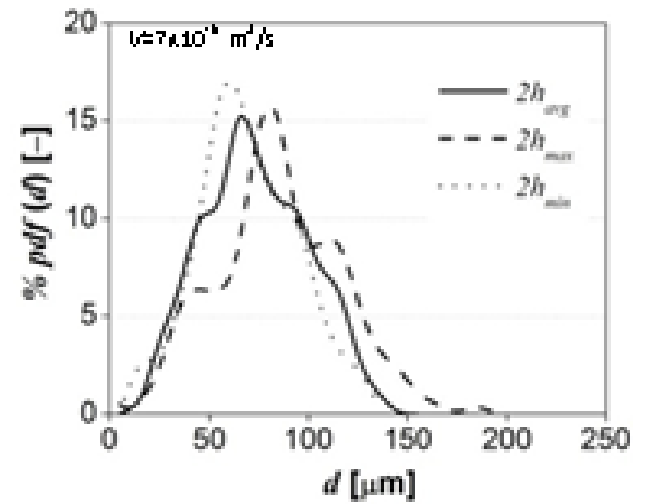
Figure 10: Probability density function distribution of drop diameter after primary break-up, function of the average, min and maximum values of the lamella thickness as predicted by 3D VOF simulations.
