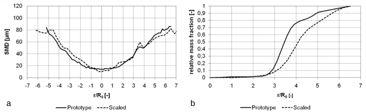
Figure 26: (a) Effect of scaling on the spray distribution at the same boundary conditions for the prototype and scaled IS; (b) comparison of relative mass fraction for (a).
