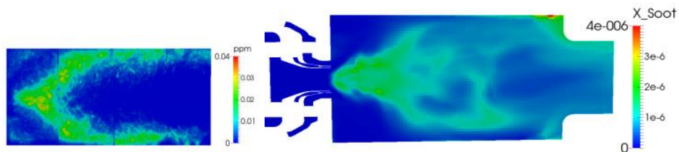
Figure 57: Measured (left) and LES results (right) soot more fraction.
