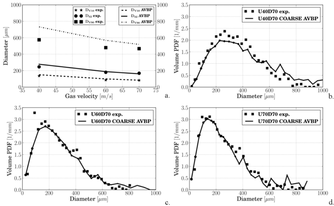
Figure 45: Characterization of the spray generated downstream the atomizing edge. Comparison between experiments (symbols) and LES (lines). a. Mean diameter versus gas velocity. b-d. Diameter distribution for three gas velocities.
