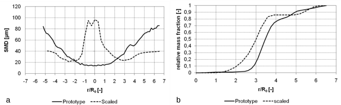
Figure 27: (a) Comparison of the two injectors at the same We-number (prototype nozzle at 3.5 % and scaled nozzle at 6.9 % pressure drops), (b) Comparison of relative mass fraction for (a).
