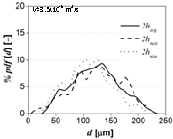
Figure 10: Probability density function distribution of drop diameter after primary break-up, function of the average, min and maximum values of the lamella thickness as predicted by 3D VOF simulations.
