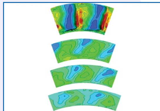
LES of fuel injector air passages
