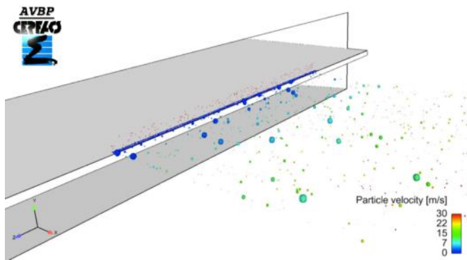
Figure 44: Instantaneous distribution of droplets downstream the atomizing edge in the KIT-ITS prefiling configuration
