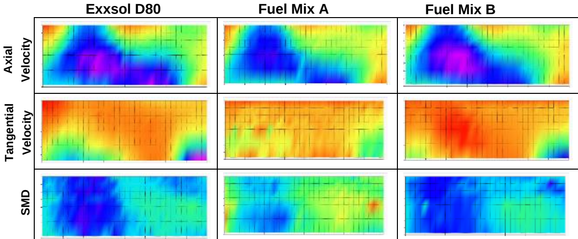
Figure 38: Comparison of alternative fuel blends using (Exxsol D80), (Fuel Mix A = 18.2% Shellsol AB; 36.3% Jet A1; 45.5% Shell GTL) and (Fuel Mix B = 25% Jet A1; Shell 75% GTL).
