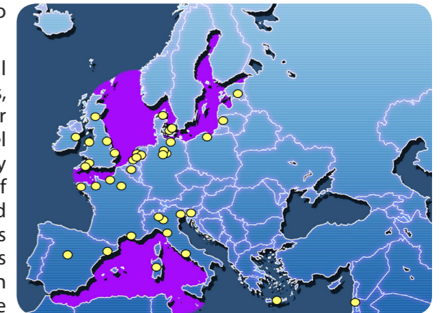
Map of Europe showing the locations of the 38 VECTORS partners (from 16 countries) and the three regional seas; the North Sea, the Baltic Sea and the western Mediterranean which are used as case study areas for the project.
