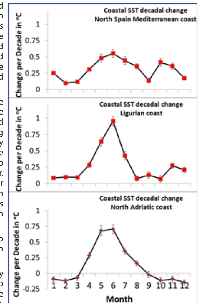
Change in SST per decade in three selected points in three regions in the western Mediterranean. Data generated from coastalwarming.com .
