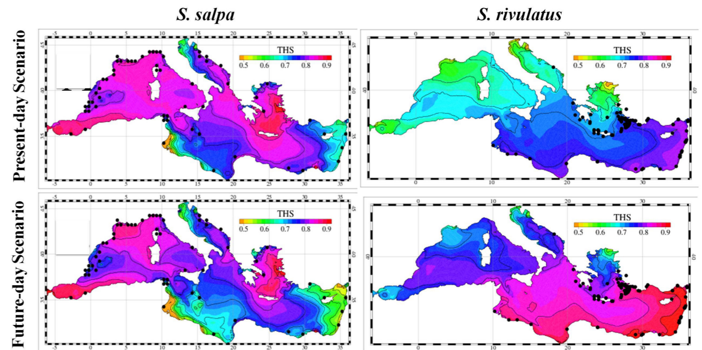
Predicting future thermal habitat suitability of competing native and invasive fish species: Thermal habitat suitability computed for the whole Mediterranean Sea from basin-scale model results. Dots represent field observations of current fish distribution for the native Sarpa salpa (a species of sea bream) and the invasive Siganus rivulatus .
