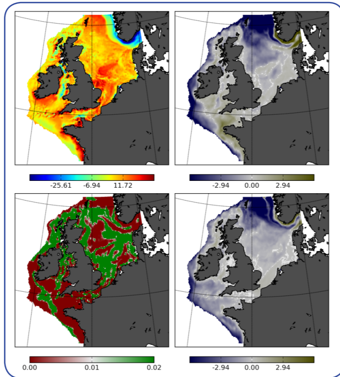
Community production for NW European shelf (mmol/m 2 ). Top Left: present day mean, Top Right: A2 change with respect to present day, Bottom Right: B1 change with respect to present day, Bottom Left: p-value of significance for difference between A2 and B1
