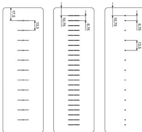
Figure 6: Sensor inserts
