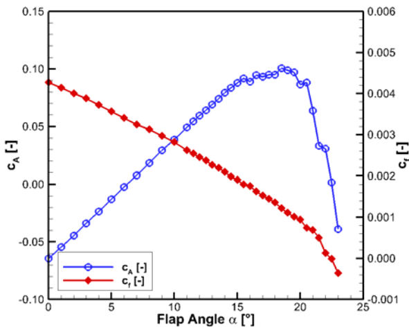
Figure 11: Lift and shear stress coefficient for u_\infty = 20 m/s
