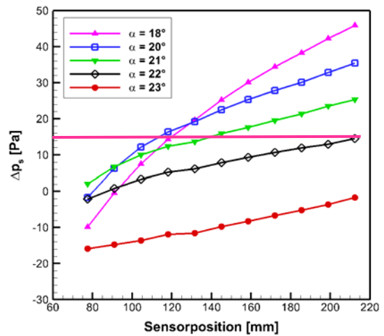
Figure 12: Pressure distribution for different flap angles
