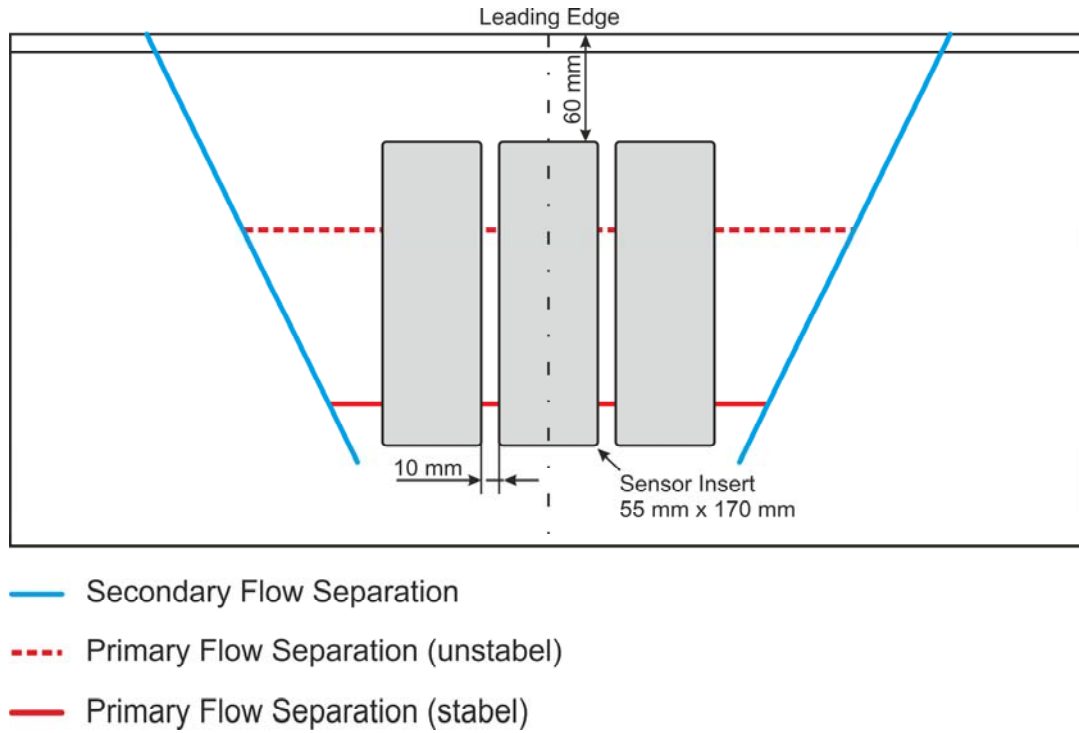
Figure 5: Sketch of the flap for the sensor tests with the results of the tuft visualisation for \alpha = 19^\circ and u_\infty = 20 \text{ m/s}
