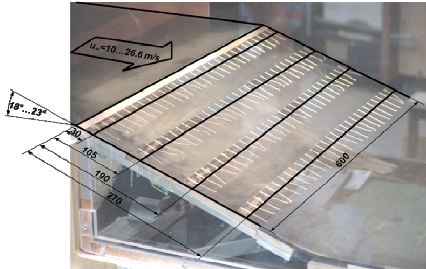
Figure 3: Experimental setup
