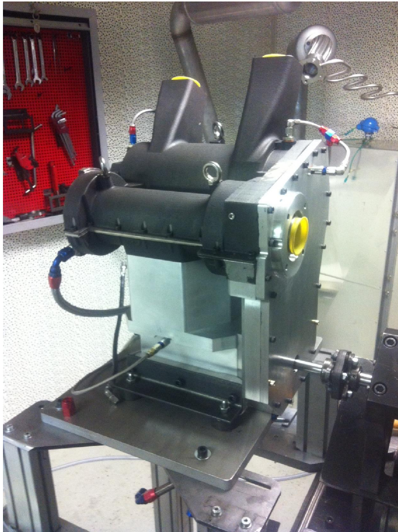
Assembled engine
