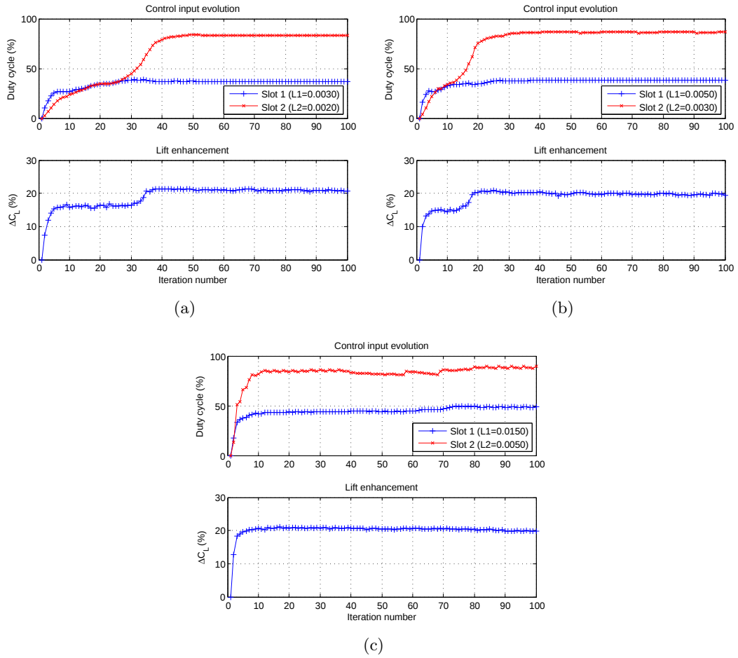
Figure A.1: Duty cycle (slot 1) vs duty cycle (slot 2)
