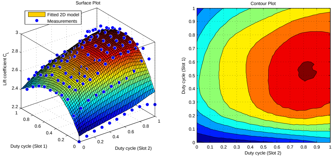
Figure 4.18: Fitted model: duty cycle 1 vs duty cycle 2.
