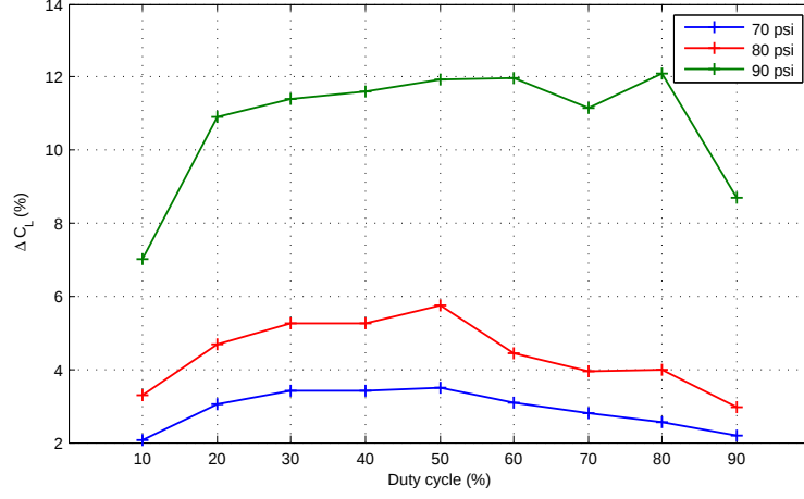
Figure 4.9: Improvement of using different duty cycles for different pressures
