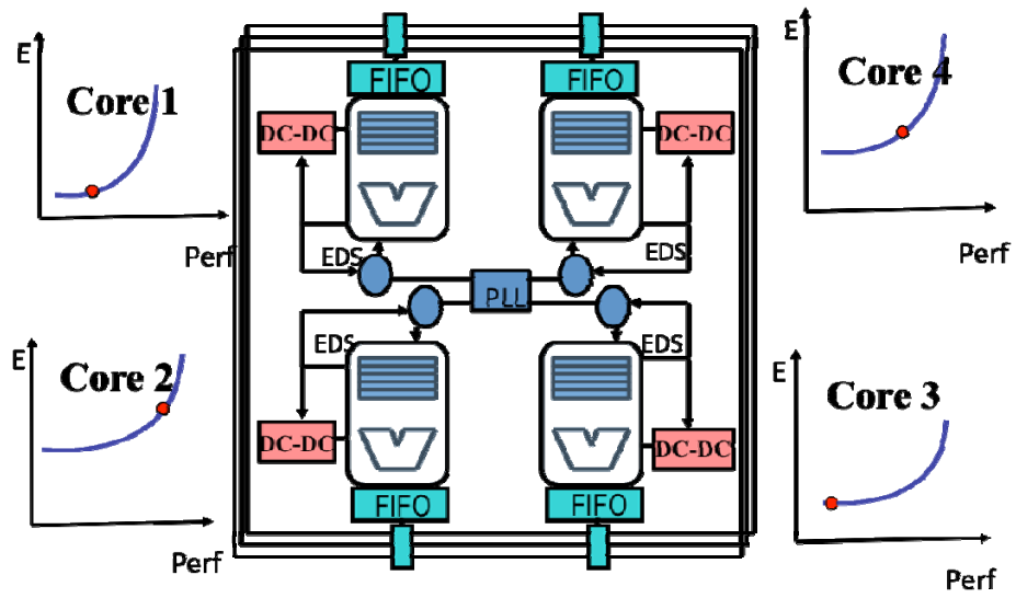
Fig. 1 DVFS for manycore processor
