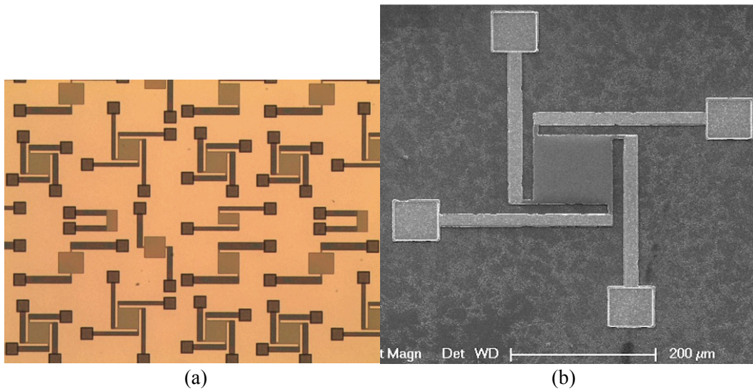
Figure 2. (a) Micrograph of the fabricated devices, (b) SEM image of a fabricated device.
