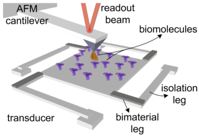
Figure 1. Conceptual drawing of an AFM cantilever engaged on a transducer in a biomolecular mechanics experiment.
