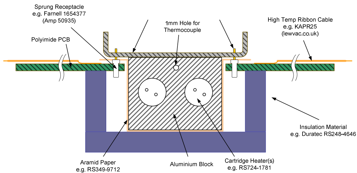
Figure Error! No text of specified style in document.-12 Electrical Demonstrator Test Interface
