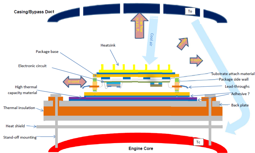
Figure Error! No text of specified style in document.-6 Schematic of Thermal Management Concepts
