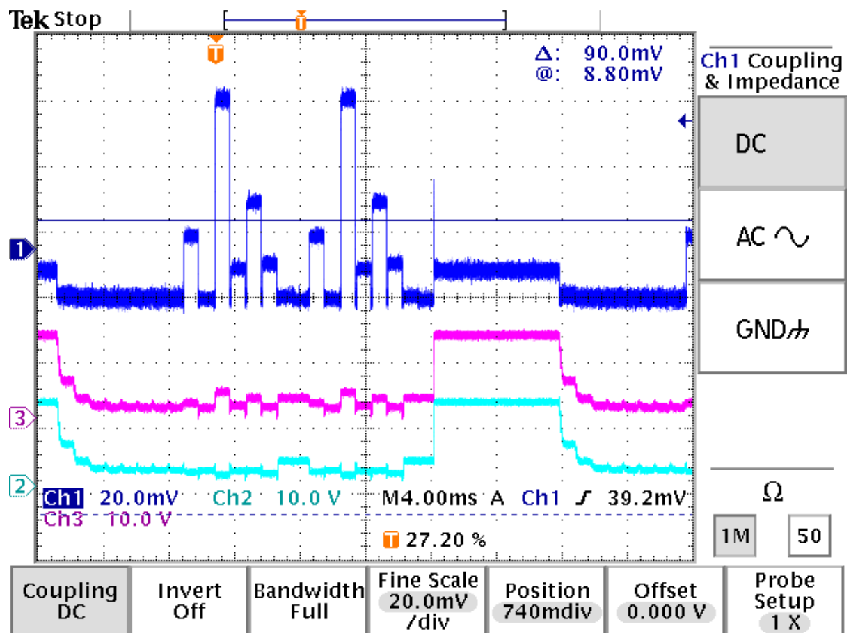
Figure Error! No text of specified style in document.-13 Electrical Demonstrator Test Waveforms at 200 °C
