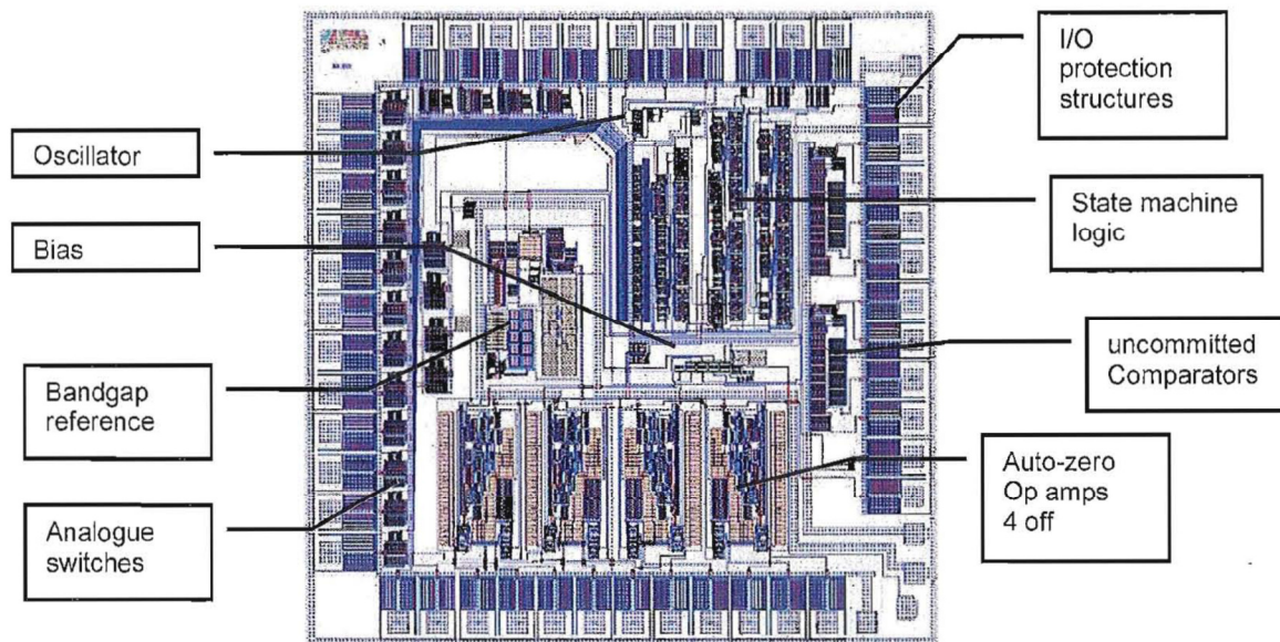
Figure Error! No text of specified style in document.-4 Final SiC IC Layout Showing Major Functional Blocks
