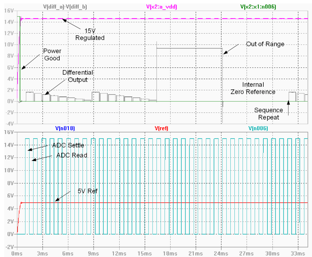
Figure Error! No text of specified style in document.-3 Simulated Waveforms of the Design Concept
