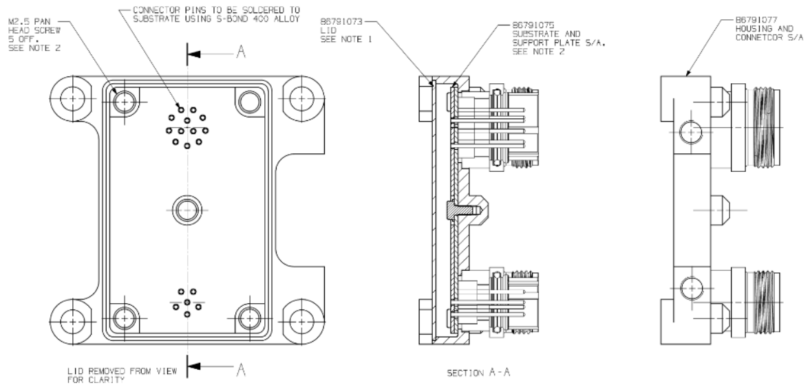
Figure Error! No text of specified style in document.-8 Mechanical Demonstrator Design (86791078)
