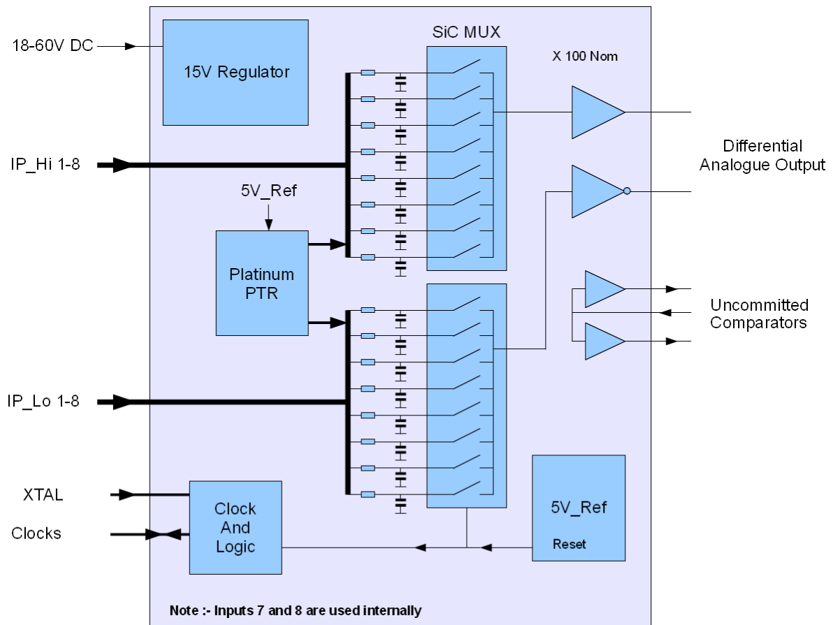
Figure Error! No text of specified style in document.-2 Proposed Data Acquisition Subsystem
