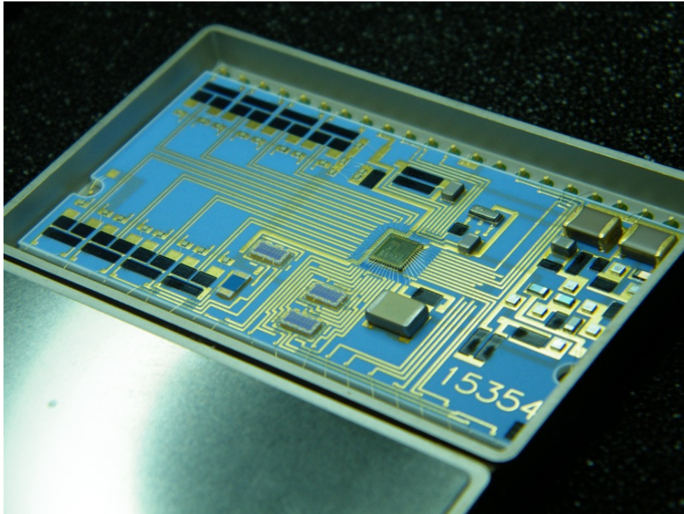
Figure Error! No text of specified style in document.-10 Electrical Demonstrator
