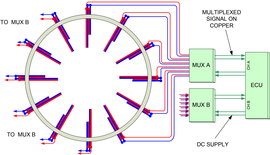
Figure Error! No text of specified style in document.-1 Multiplexed TGT Measurement
