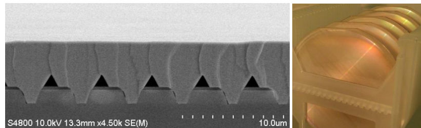
SEM image of coalesced layer of GaN producing a (11-22) surface and a batch of 100mm diameter (11-22) templates
