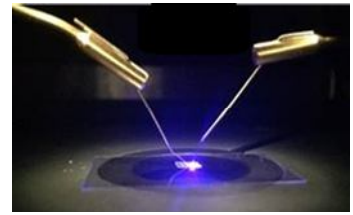
50 \mu\text{m} thick free standing semipolar LED fabricated by laser lift-off that has demonstrated a 30% improvement in light output through the backside of the LED when compared to LEDs without substrate
