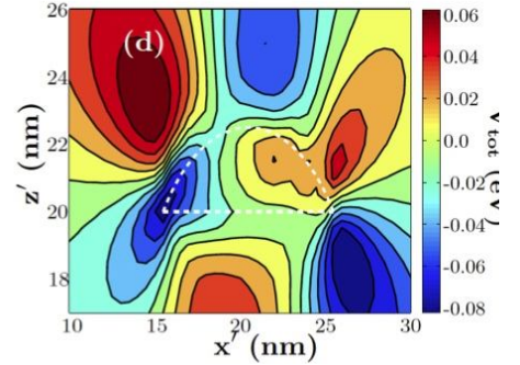
Built-in potential V_{tot} in a semipolar (11-22) InGaIn quantum dot. V_{tot} is shown for a slice through the centre of the structure
