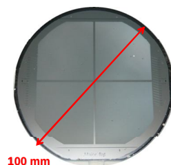
100 mm patterned (113) Si wafer with 4.5 \mu\text{m} of un-cracked semi-polar GaN.
