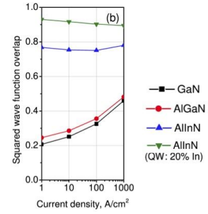
Semipolar In_{0.17}Ga_{0.83}N -based LED designed for blue emission (450 nm): Calculated ground state electron and hole wavefunction overlap for structures containing GaN, AlGaIn and AlInN barriers.
