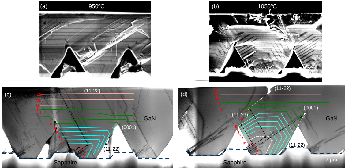
Cross-sectional view of samples with the GaN layer before coalescence grown at 950°C and 1050°C. (a,b) SEM images, where the Si-doped GaN marker layers are visible. (c,d) STEM images with the marker layers redrawn corresponding to those in (a,b). The blue lines are associated with the GaN layer grown at 950°C or 1050°C. The surface of the pre-structured sapphire substrates is marked by dashed dark blue lines. The position of a SiN interlayer is marked by red dashed lines, which was deposited at an early stage of the growth to block the propagation of dislocations along the c -direction. The black arrows indicate the bending of dislocations when they meet the (11-22) facet.
