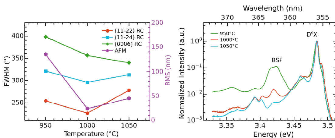
Left: FWHM of HRXRD rocking curves and surface roughness measured by AFM against growth temperature of the pre-coalesced stripe. Right: Low temperature ( T=15\text{K} ) PL spectra.
