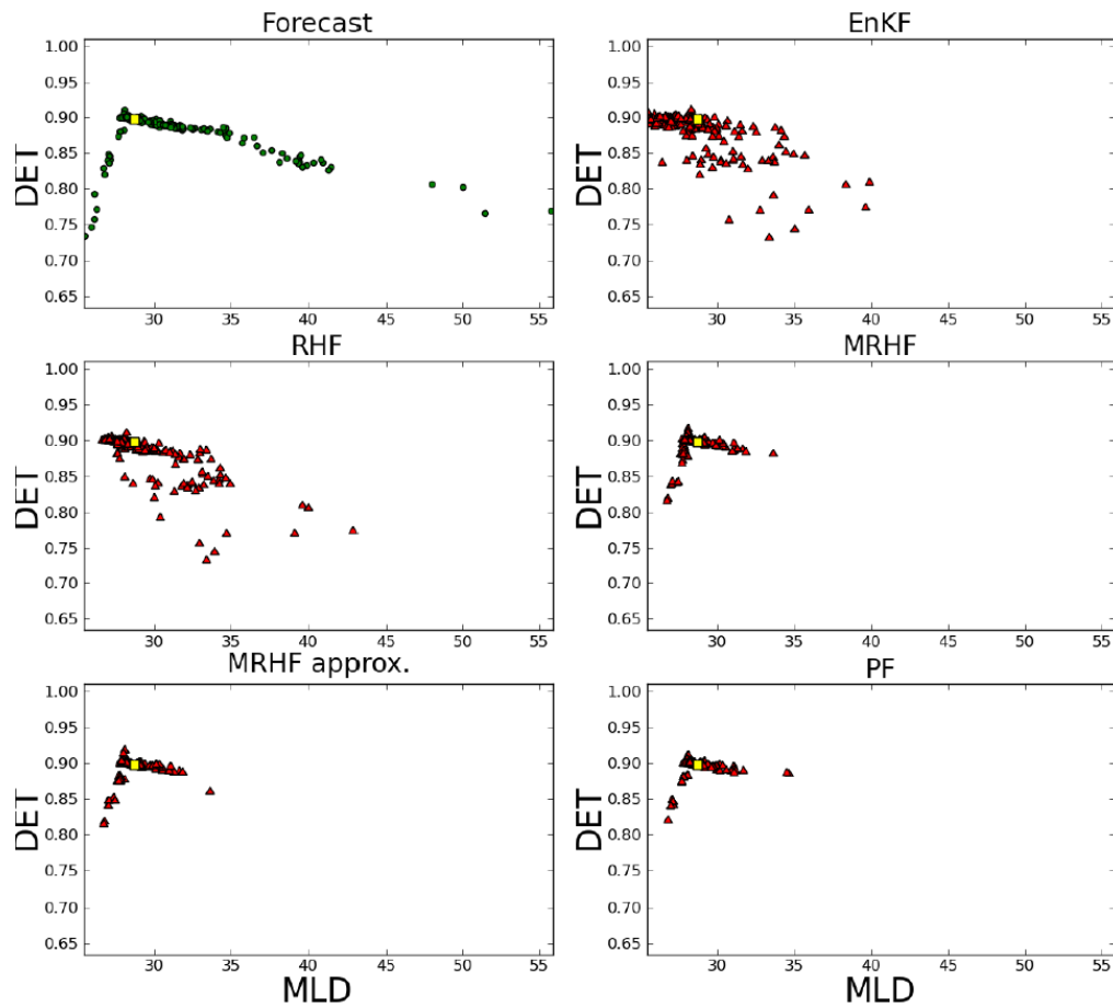
Figure 2.2: Application of the MRHF to the NATL025 implementation with bio-chemical model. Chl is observed and mixed layer depth and detritus are analysed. The members of the MRHF with or without the approximation in the joint probabilities work very well in this case.
