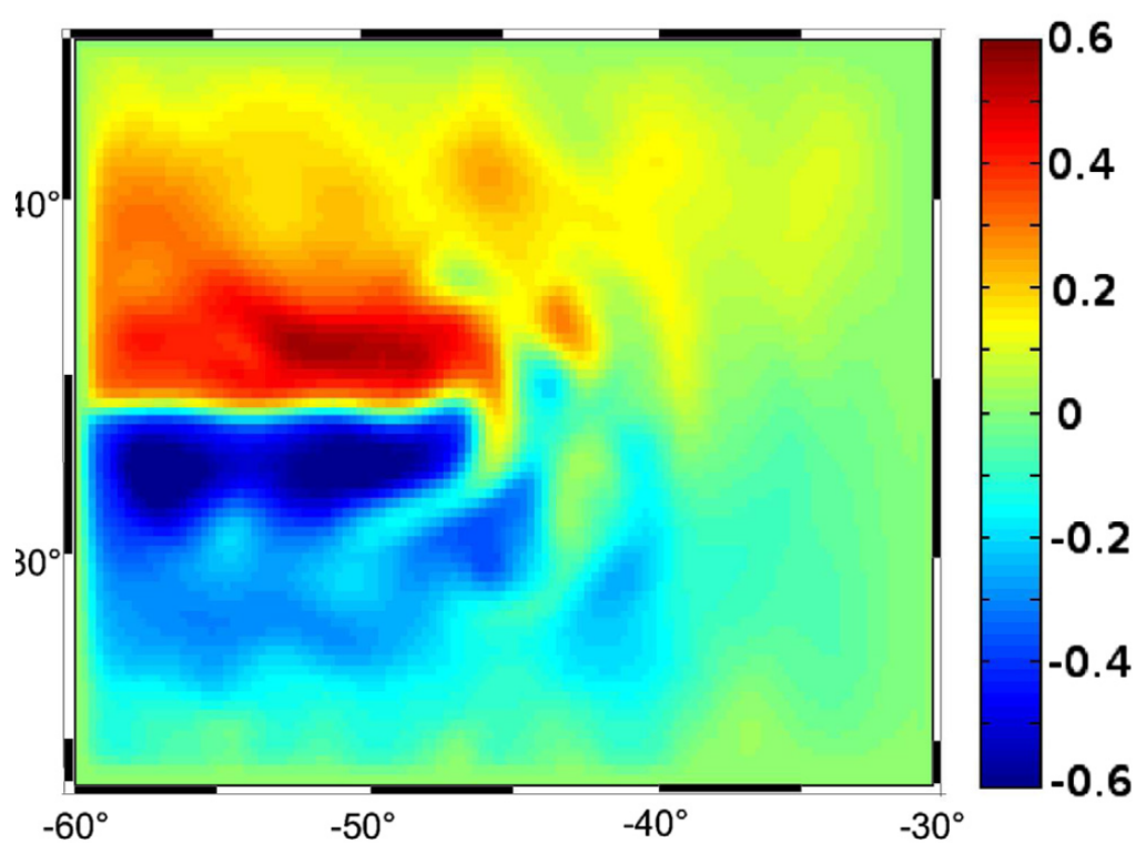
Figure 2.5: Snapshot of SSH in the medium-size benchmark.
