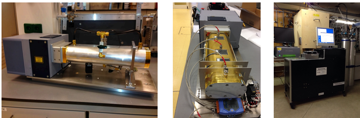
Figure 1.3.5: Spectronus aluminum measurement cell (and Bruker IR Cube FTIR detector (in gray/black)) before (left) and after (middle) upgrade of cell by braising, gold plating and implementing improved temperature control. Right: Spectronus instrument at the Cabauw control room.
