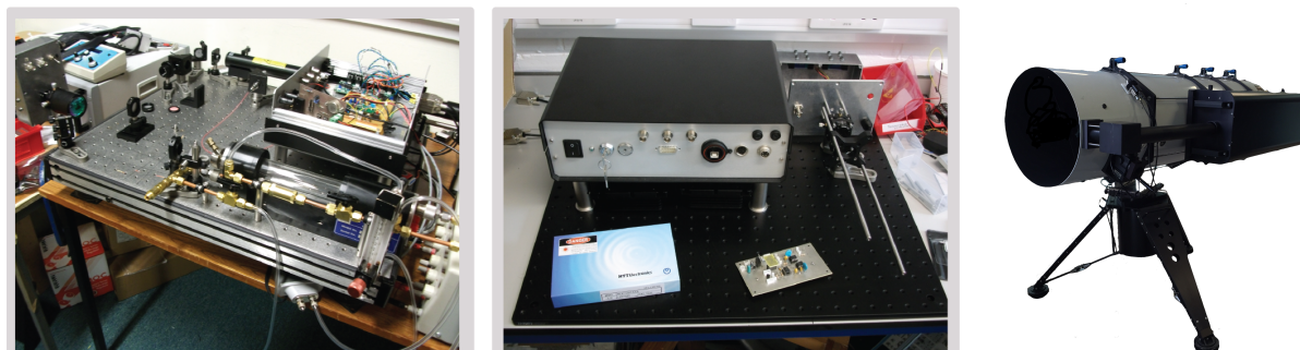
Figure 1.3.6: Seed modules (CO 2 on the left, CH 4 in the middle) for DIAL of greenhouse gases, a photograph on the right of the Mark 2 DIAL with the laser attached to the tripod-mounted Newtonian telescope
