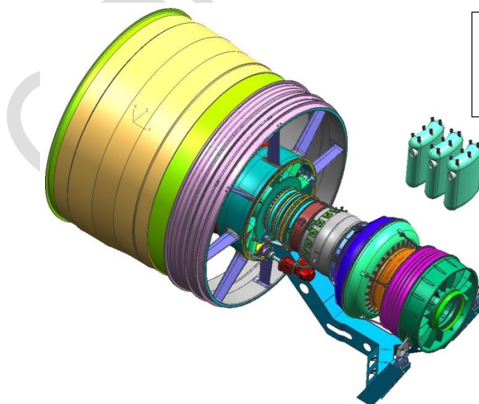
Figure 2.3.3. General isometric view of the AHEAD CRF hybrid engine with Heat Exchangers modules positioned outside engine.
