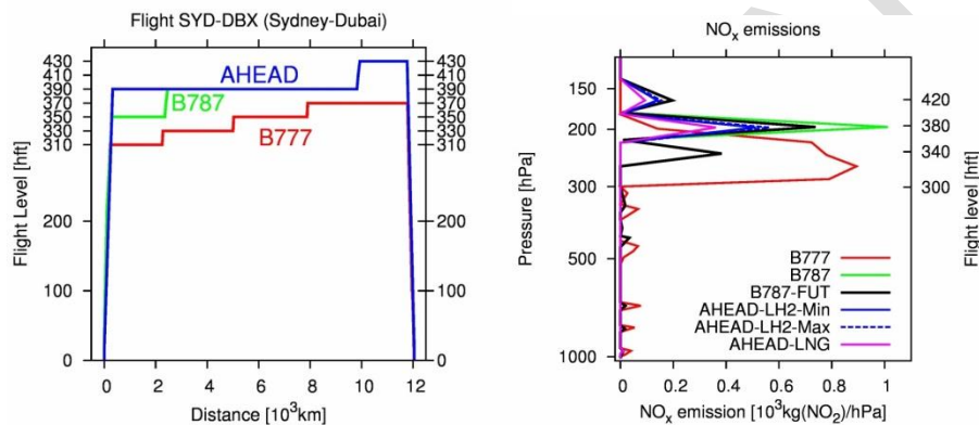
Fig. 2.7.1. Left: Flight profiles for the route Sydney to Dubai; Right: Annual global mean emission profile for nitrogen oxides.
