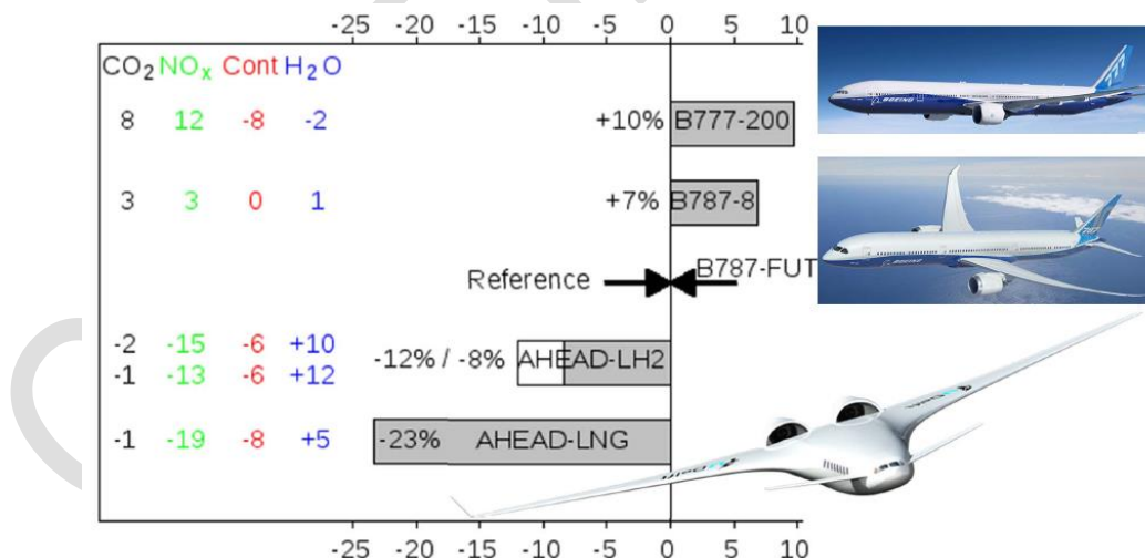
Fig. 2.7.3. Overall climate impact assessment: Relative change in the 100 year-mean future temperature change (%) for the individual aircraft scenarios (identical to relative change in equivalent \text{CO}_2 – eq \text{CO}_2 emission). B787-FUT is taken as a reference. Total relative changes are shown at the bars, the contribution (%) from different emissions are added on the left. The sum equals the totals, though rounding errors might occur.
