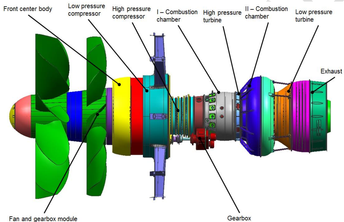
Figure 2.3.4. AHEAD CRF hybrid engine modules review.
