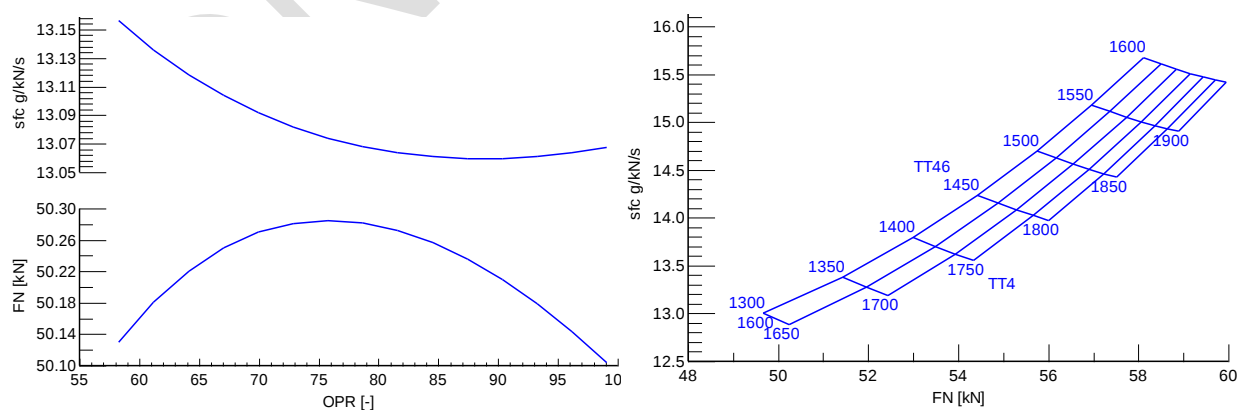
Figure 2.2.5: The variation of SFC and FN various design parameters.
