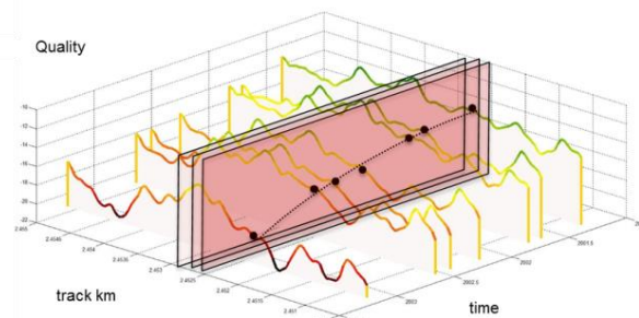
Figure 1-5 Generation of track deterioration profiles.
