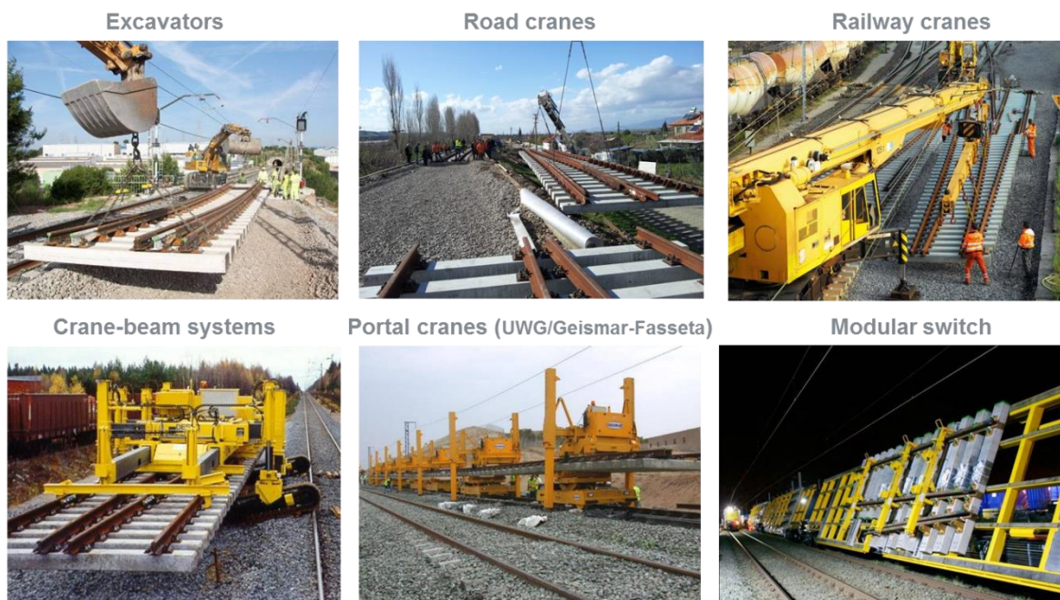
Figure 1-9 Different techniques for track renewal.
