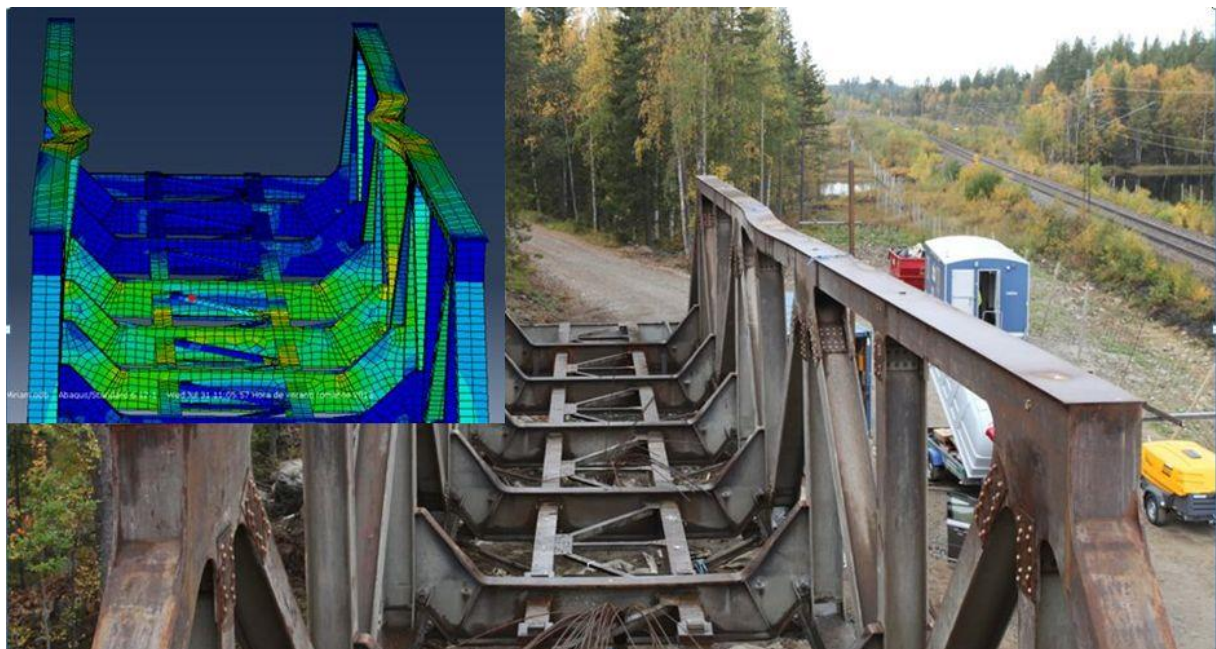
Figure 1-4 The Åby bridge after failure, which was caused by buckling of the top flange of the main truss girders. The failure was quite ductile and the bridge could continue to carry a high load after failure, as predicted by the FEM model of the failure, shown in insert.
