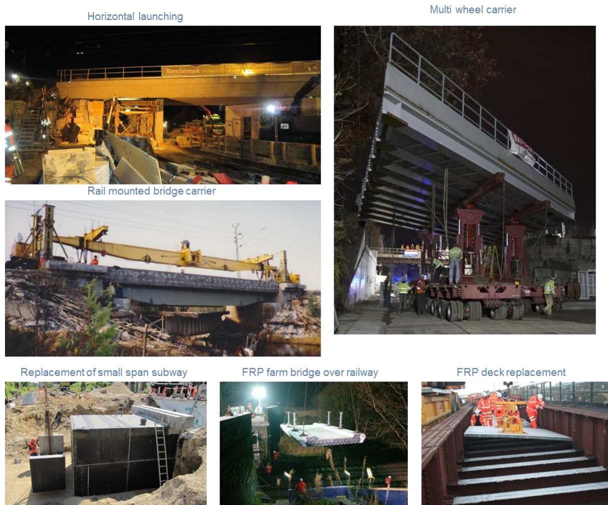
Figure 1-8 Example of bridge replacement methods
