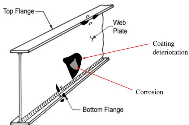
Figure 1-6 Generation of metallic bridge deterioration profiles.
