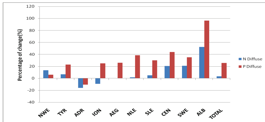
Figure 17 Expected changes in diffuse emissions of Nitrogen and Phosphorus (N diffuse and P diffuse respectively) by the year 2030, according to the Adapting Mosaic (AM) scenario, in the different Mediterranean sub-basins*.
