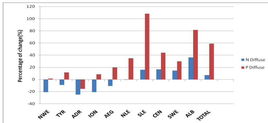
Figure 18 Expected changes in diffuse emissions of Nitrogen and Phosphorus (N diffuse and P diffuse respectively) by the year 2030, according to the Technogarden (TG) scenario, in the different Mediterranean sub-basins*.
