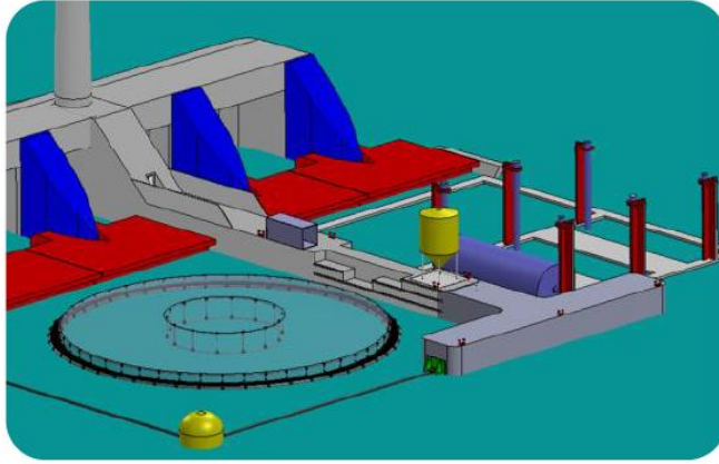
Figure 13. WEC with attached fish cages
