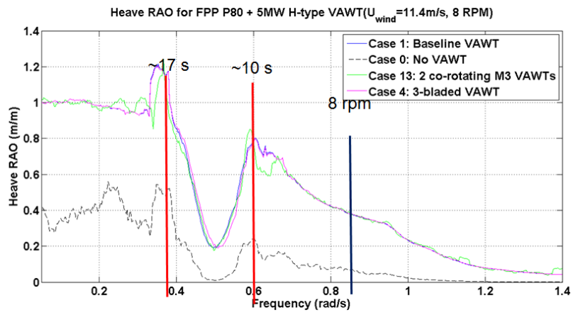
Figure 19. Heave response with different VAWT configurations (number of turbines and number of blades)
