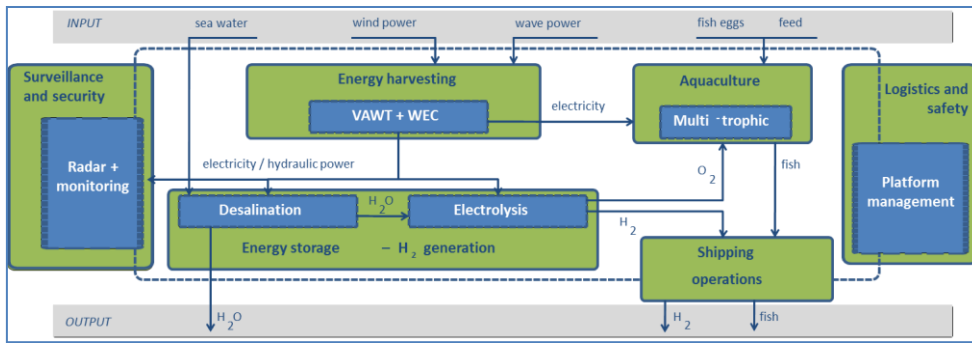
Figure 2. Process Flow Diagram showing integrations of activities in the H2OCEAN design
