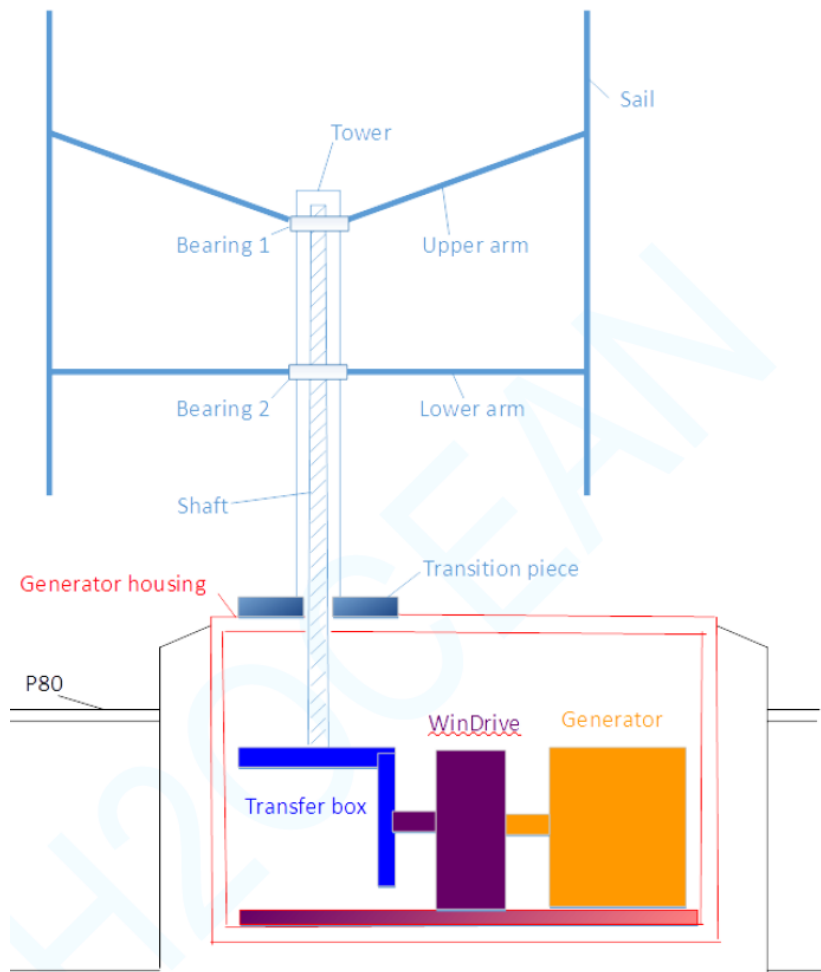
Figure 21. Coupling of the VAWT shaft with a generator using a 90° transfer box
