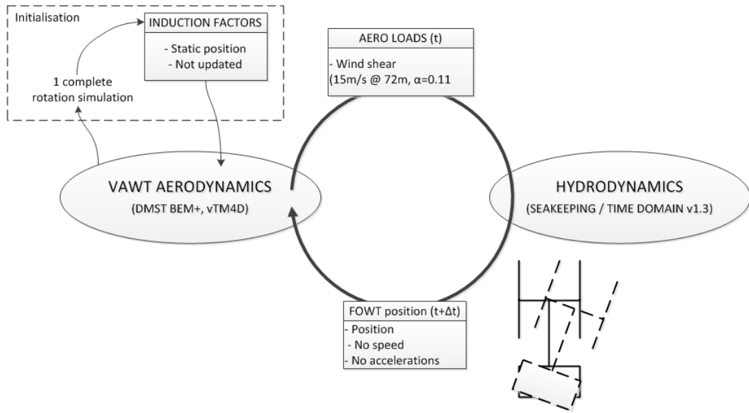
Figure 22. FloVAWT semi-coupled model scheme
