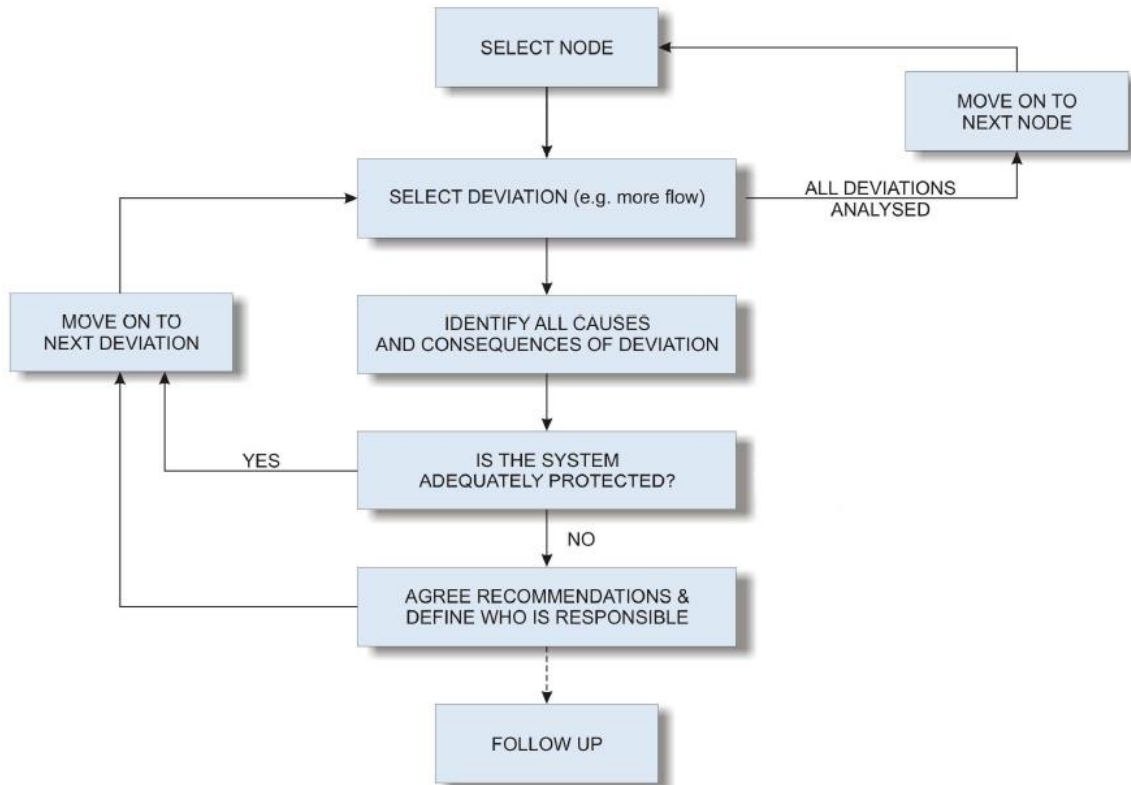
Figure 23. HAZOP Process Flowchart
