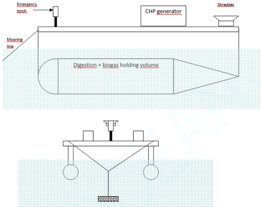
Figure 25. FAD arrangement and layout1
