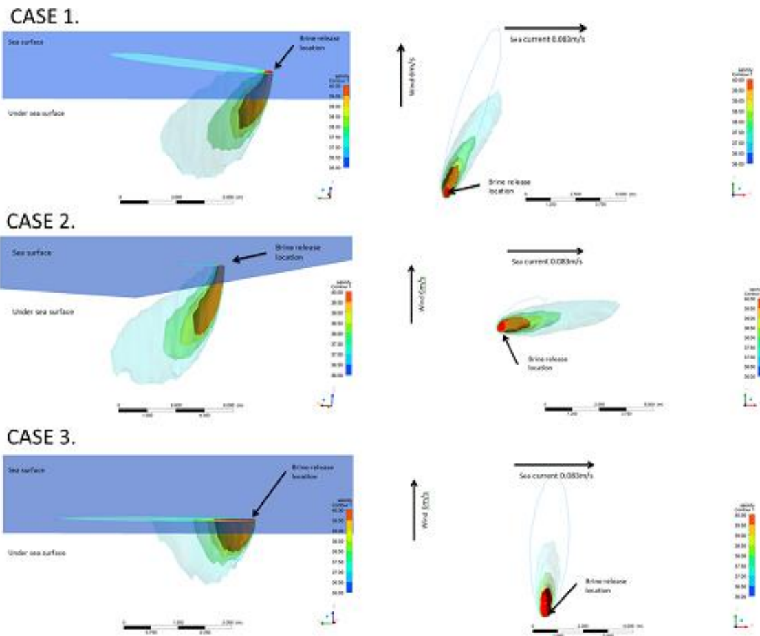
Figure 29. Three case studies of the salinity plume behavior
