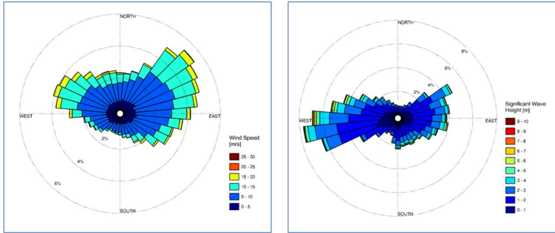
Figure 3. Wind rose for the Portuguese Site
