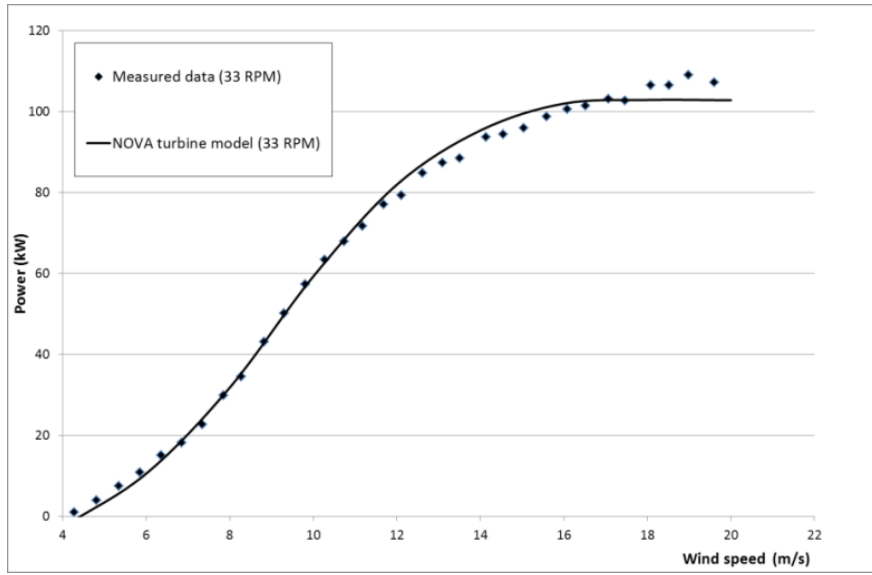
Figure 5. Predicted Power of the VAWT-260 H-rotor
