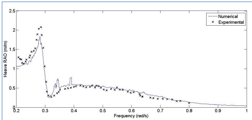
Figure 6. Validation of heave RAO, numerical results VS experimental (22), GVA 4000 semi-submersible
