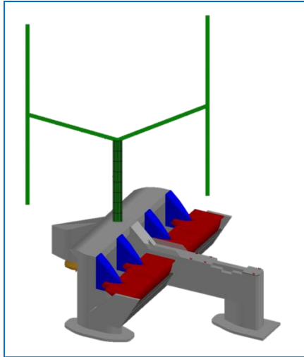
Figure 7. Initial concept of the hybrid VAWT-WEC device
