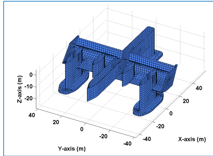
Figure 8. Surface mesh for the P80 WEC required for the hydrodynamic design
