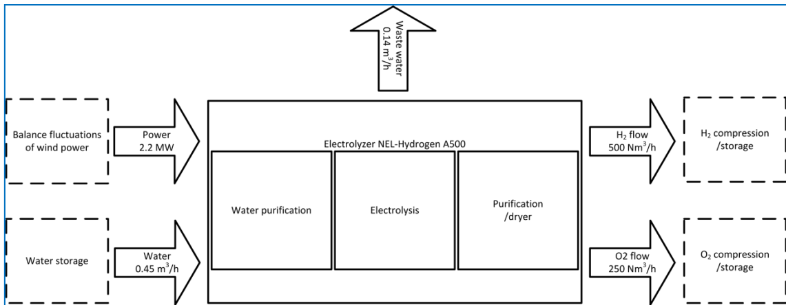
Figure 9. Process diagram for a single electrolyser unit – using specifications from alkaline electrolyser unit A500 from NEL Hydrogen as a base.
