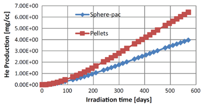
Figure 12 : Predicted helium production of the Am-BB fuel based on MCNP/FISPACT burn-up calculations
